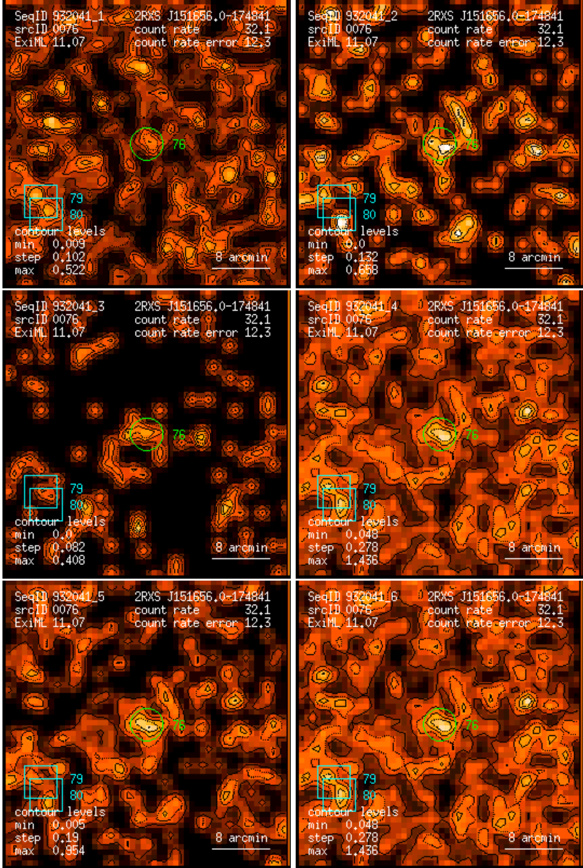
Figure 76: RASS 932041: detection 0076: band rate images, Gaussian filter: (1) PSPC channels 11 – 41, (2) 52 – 90, (3) 91 – 201, (4) 11 – 235, (5) 52 – 201, (6) 11 – 201. Broad band rates in counts/ks. Band rate contour levels in counts/ks/arcmin 2 .
