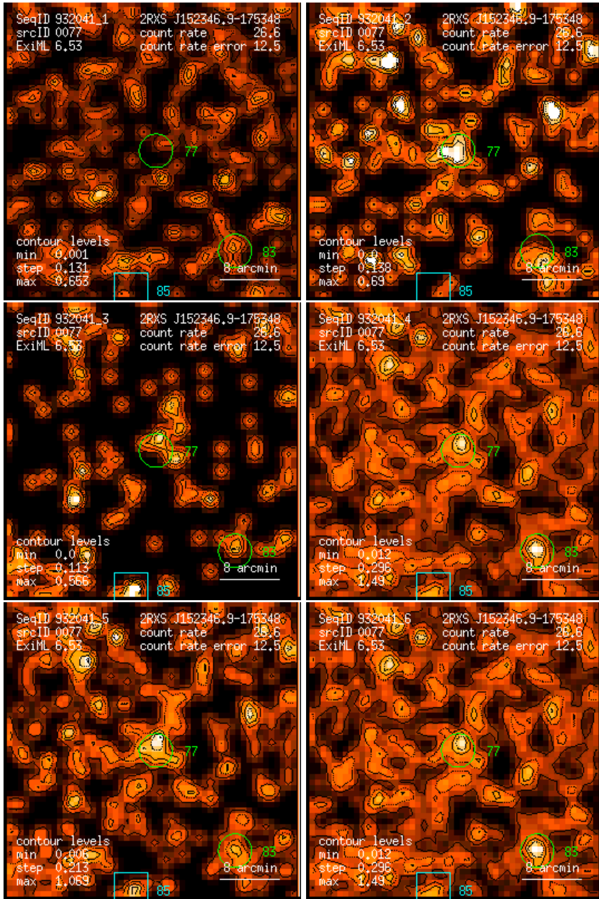
Figure 77: RASS 932041: detection 0077: band rate images, Gaussian filter: (1) PSPC channels 11 – 41, (2) 52 – 90, (3) 91 – 201, (4) 11 – 235, (5) 52 – 201, (6) 11 – 201. Broad band rates in counts/ks. Band rate contour levels in counts/ks/arcmin 2 .
