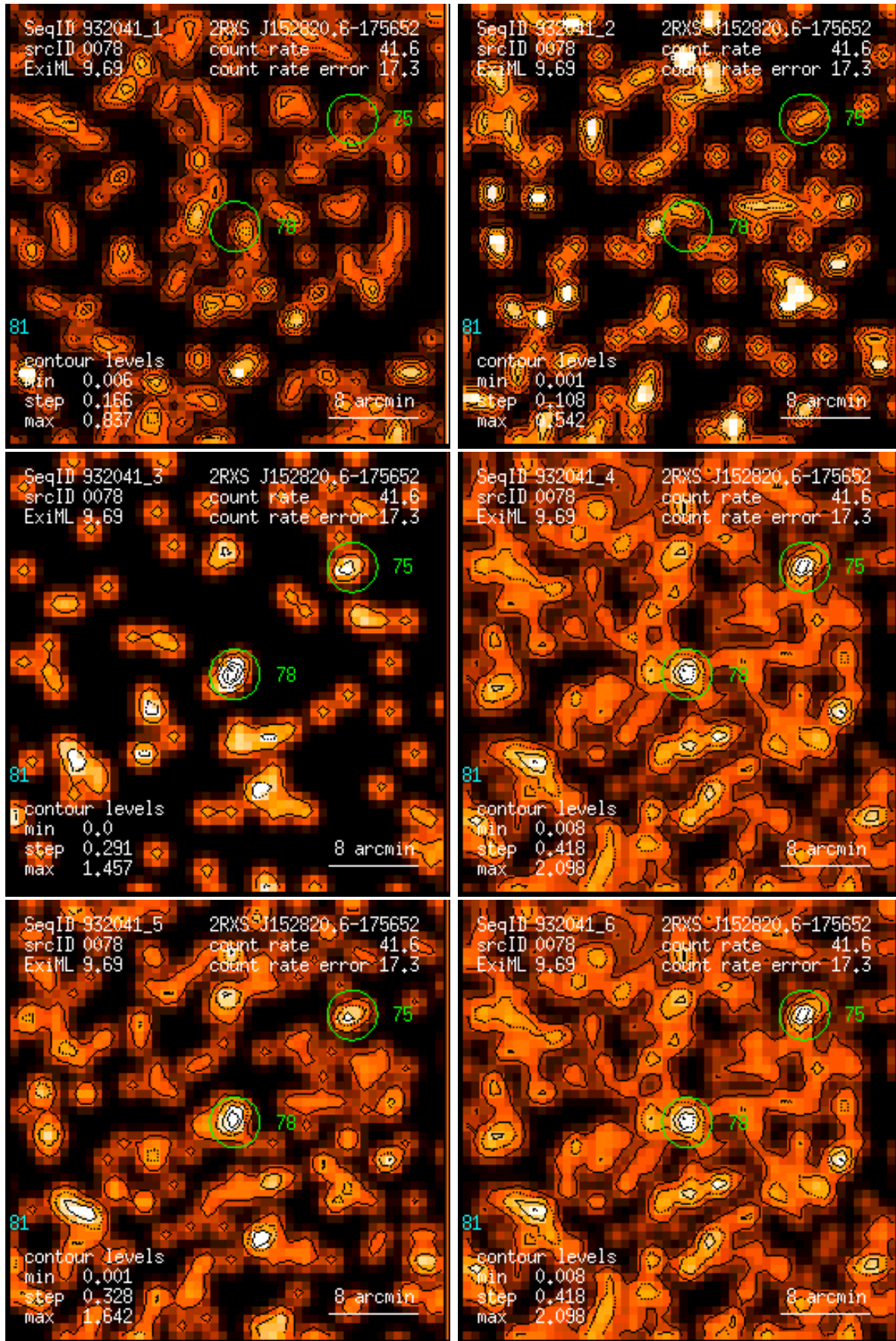
Figure 78: RASS 932041: detection 0078: band rate images, Gaussian filter: (1) PSPC channels 11 – 41, (2) 52 – 90, (3) 91 – 201, (4) 11 – 235, (5) 52 – 201, (6) 11 – 201. Broad band rates in counts/ks. Band rate contour levels in counts/ks/arcmin 2 .
