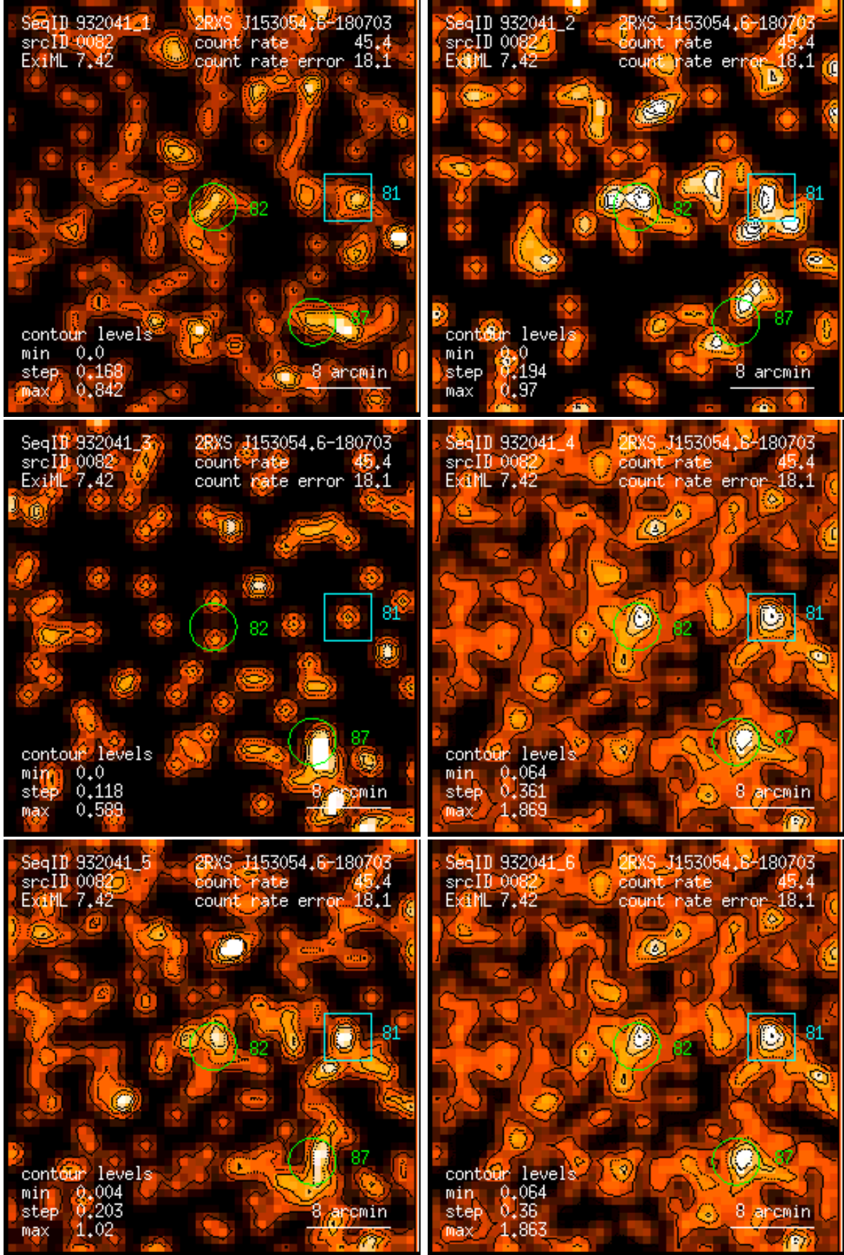
Figure 82: RASS 932041: detection 0082: band rate images, Gaussian filter: (1) PSPC channels 11 – 41, (2) 52 – 90, (3) 91 – 201, (4) 11 – 235, (5) 52 – 201, (6) 11 – 201. Broad band rates in counts/ks. Band rate contour levels in counts/ks/arcmin 2 .
