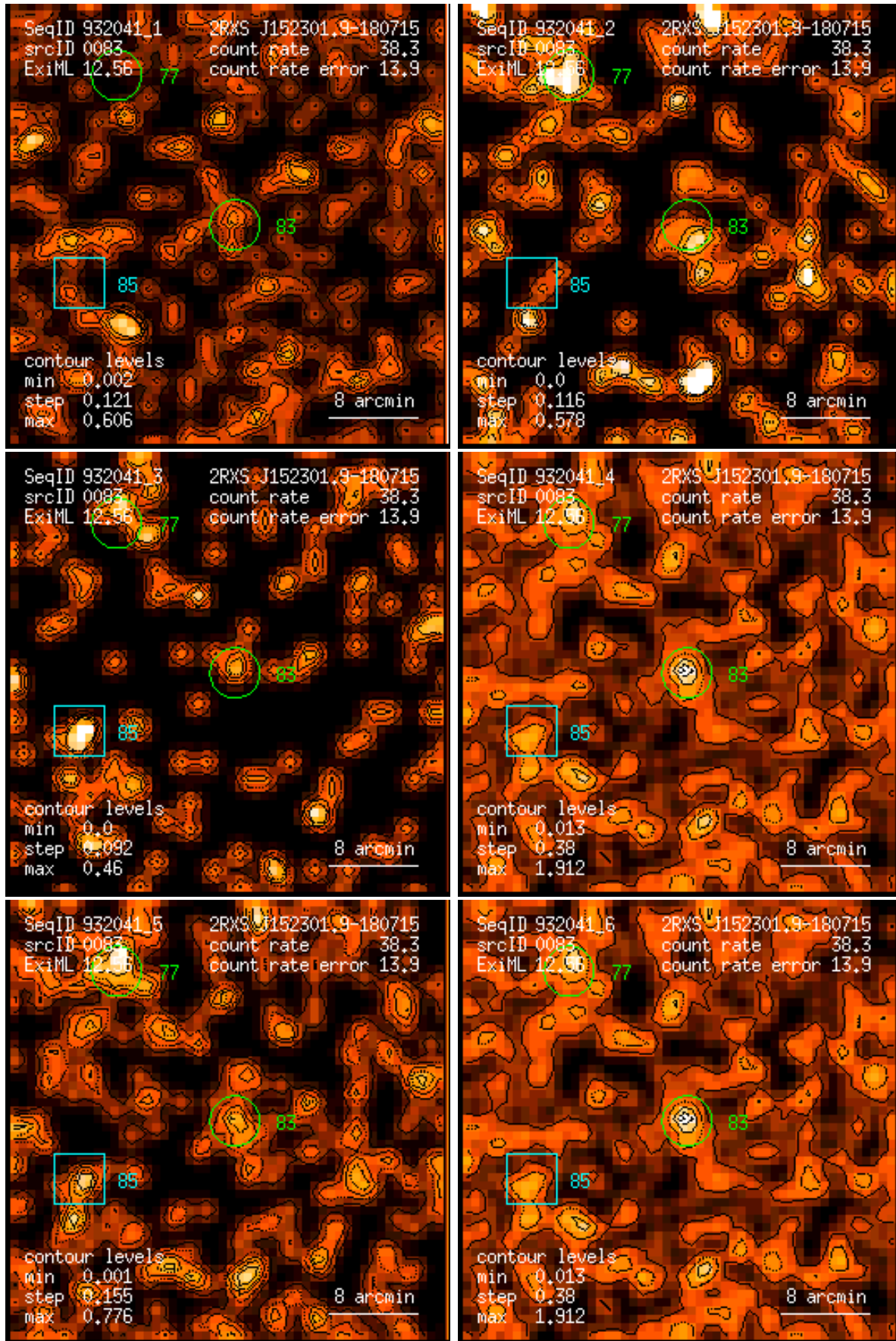
Figure 83: RASS 932041: detection 0083: band rate images, Gaussian filter: (1) PSPC channels 11 – 41, (2) 52 – 90, (3) 91 – 201, (4) 11 – 235, (5) 52 – 201, (6) 11 – 201. Broad band rates in counts/ks. Band rate contour levels in counts/ks/arcmin 2 .
