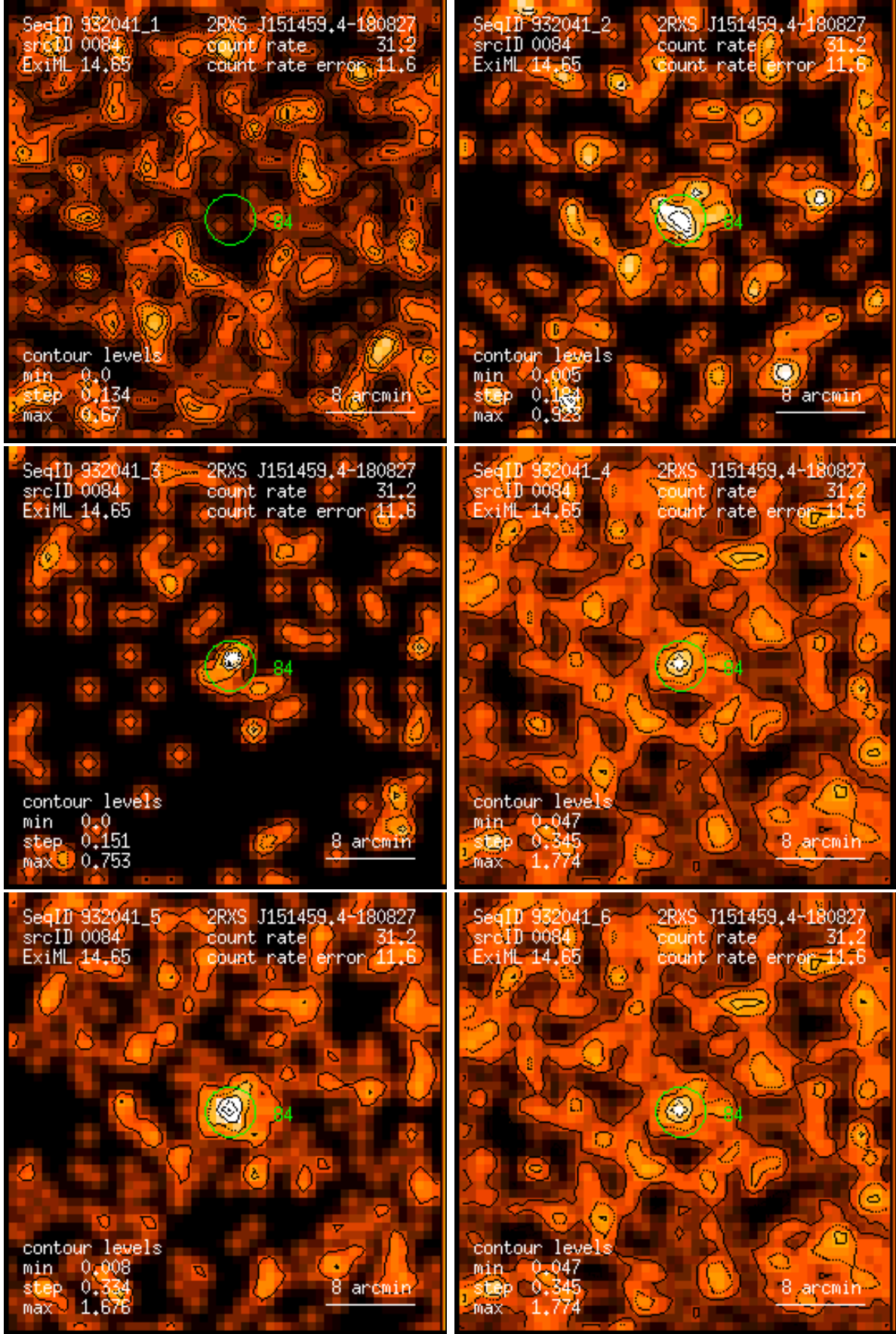
Figure 84: RASS 932041: detection 0084: band rate images, Gaussian filter: (1) PSPC channels 11 – 41, (2) 52 – 90, (3) 91 – 201, (4) 11 – 235, (5) 52 – 201, (6) 11 – 201. Broad band rates in counts/ks. Band rate contour levels in counts/ks/arcmin 2 .
