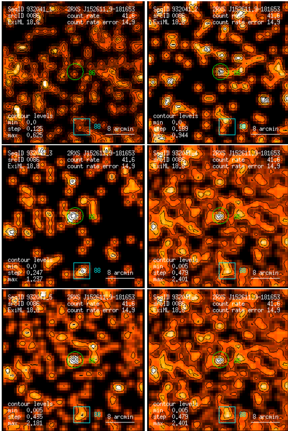
Figure 86: RASS 932041: detection 0086: band rate images, Gaussian filter: (1) PSPC channels 11 – 41, (2) 52 – 90, (3) 91 – 201, (4) 11 – 235, (5) 52 – 201, (6) 11 – 201. Broad band rates in counts/ks. Band rate contour levels in counts/ks/arcmin 2 .
