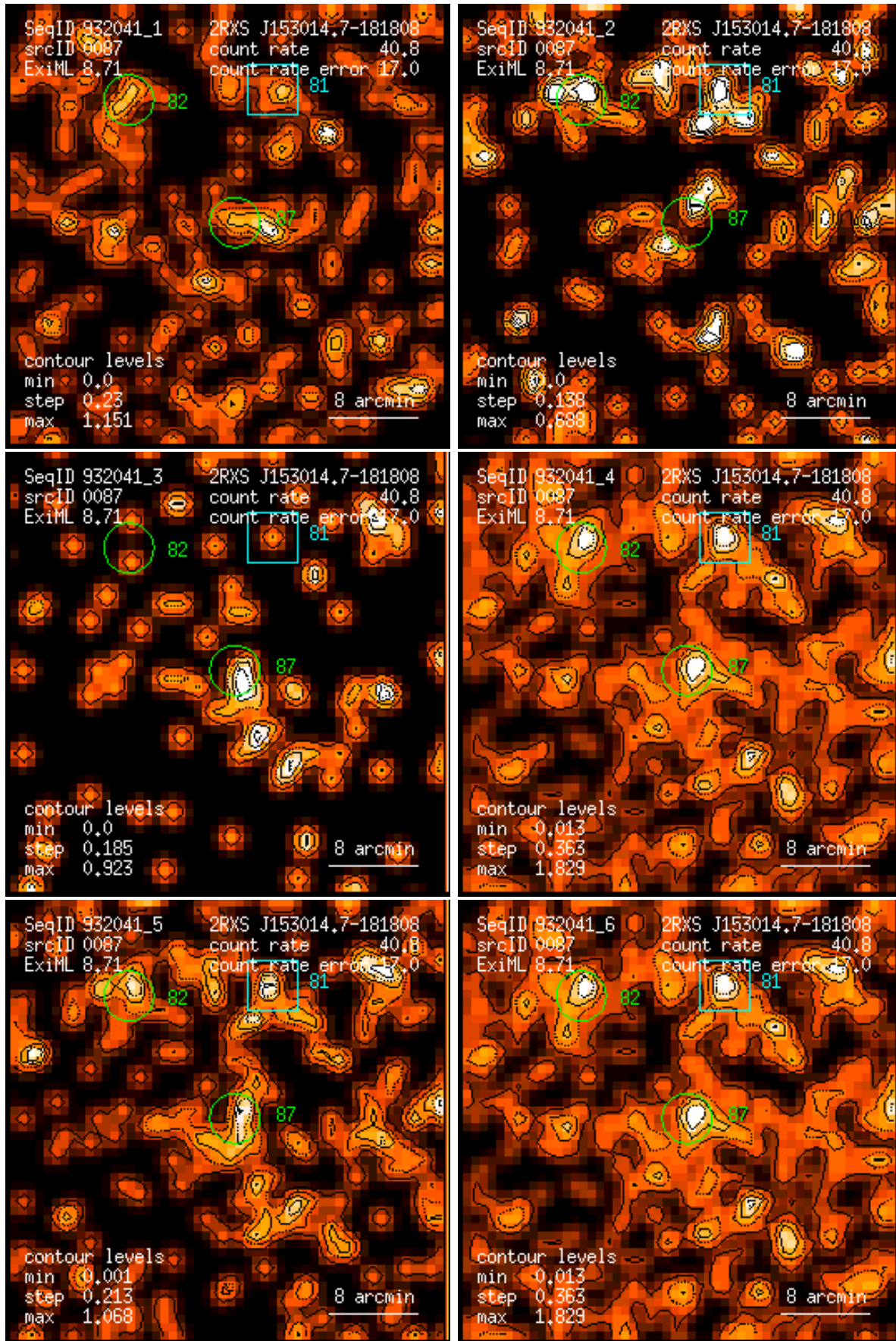
Figure 87: RASS 932041: detection 0087: band rate images, Gaussian filter: (1) PSPC channels 11 – 41, (2) 52 – 90, (3) 91 – 201, (4) 11 – 235, (5) 52 – 201, (6) 11 – 201. Broad band rates in counts/ks. Band rate contour levels in counts/ks/arcmin 2 .
