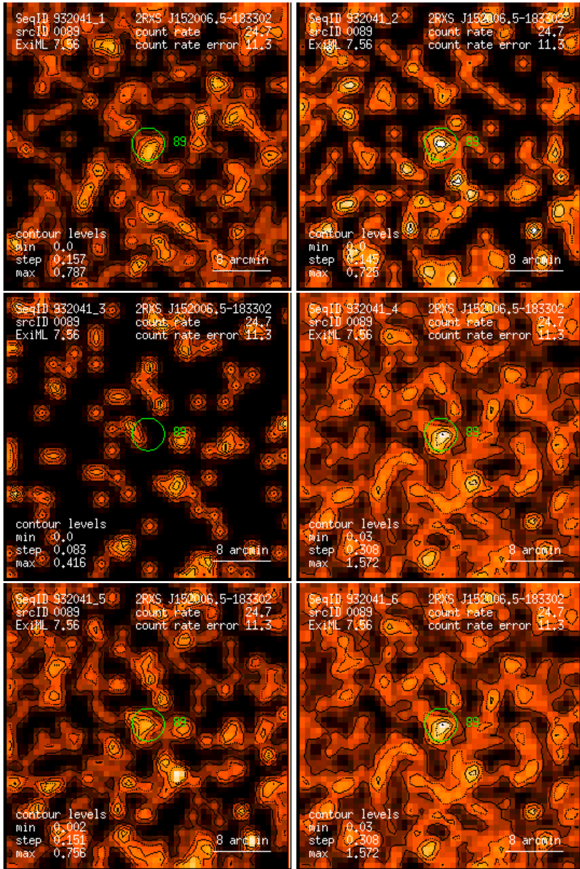
Figure 89: RASS 932041: detection 0089: band rate images, Gaussian filter: (1) PSPC channels 11 – 41, (2) 52 – 90, (3) 91 – 201, (4) 11 – 235, (5) 52 – 201, (6) 11 – 201. Broad band rates in counts/ks. Band rate contour levels in counts/ks/arcmin 2 .
