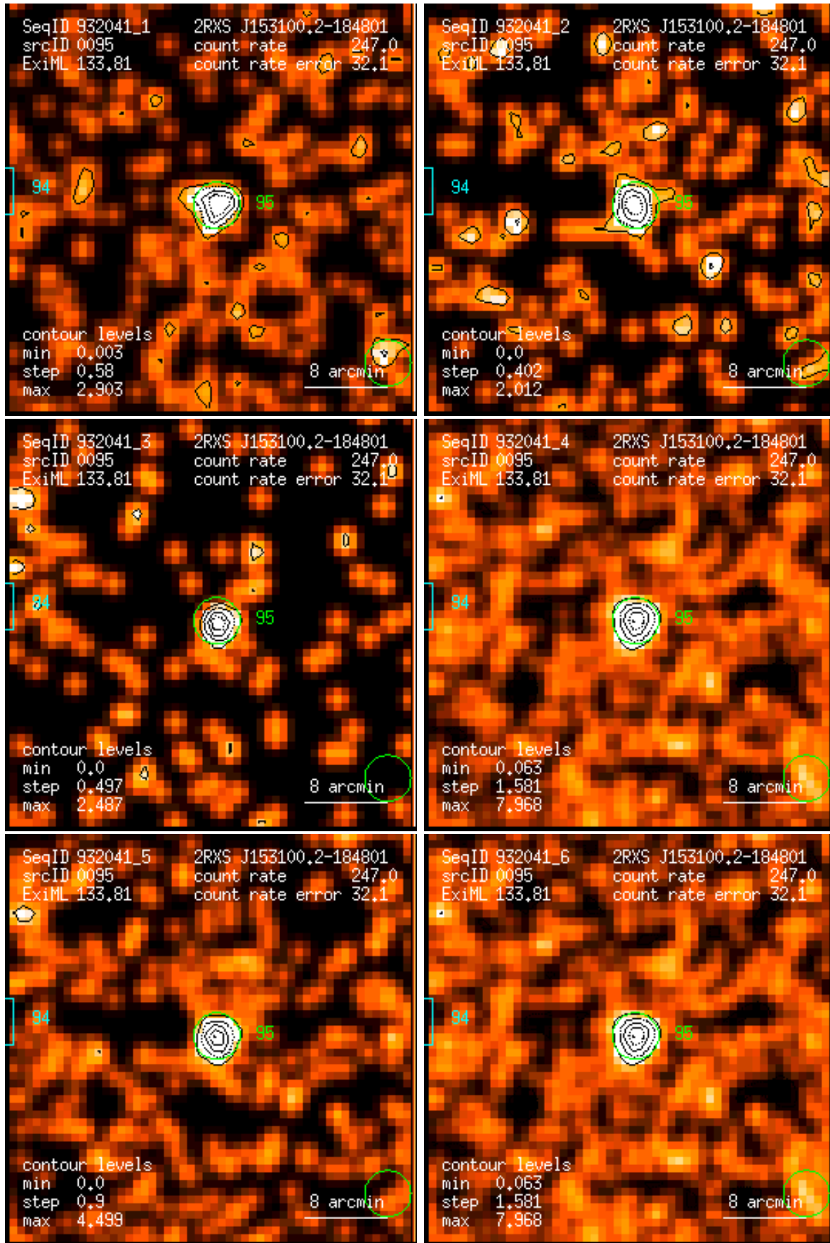
Figure 95: RASS 932041: detection 0095: band rate images, Gaussian filter: (1) PSPC channels 11 – 41, (2) 52 – 90, (3) 91 – 201, (4) 11 – 235, (5) 52 – 201, (6) 11 – 201. Broad band rates in counts/ks. Band rate contour levels in counts/ks/arcmin 2 .
