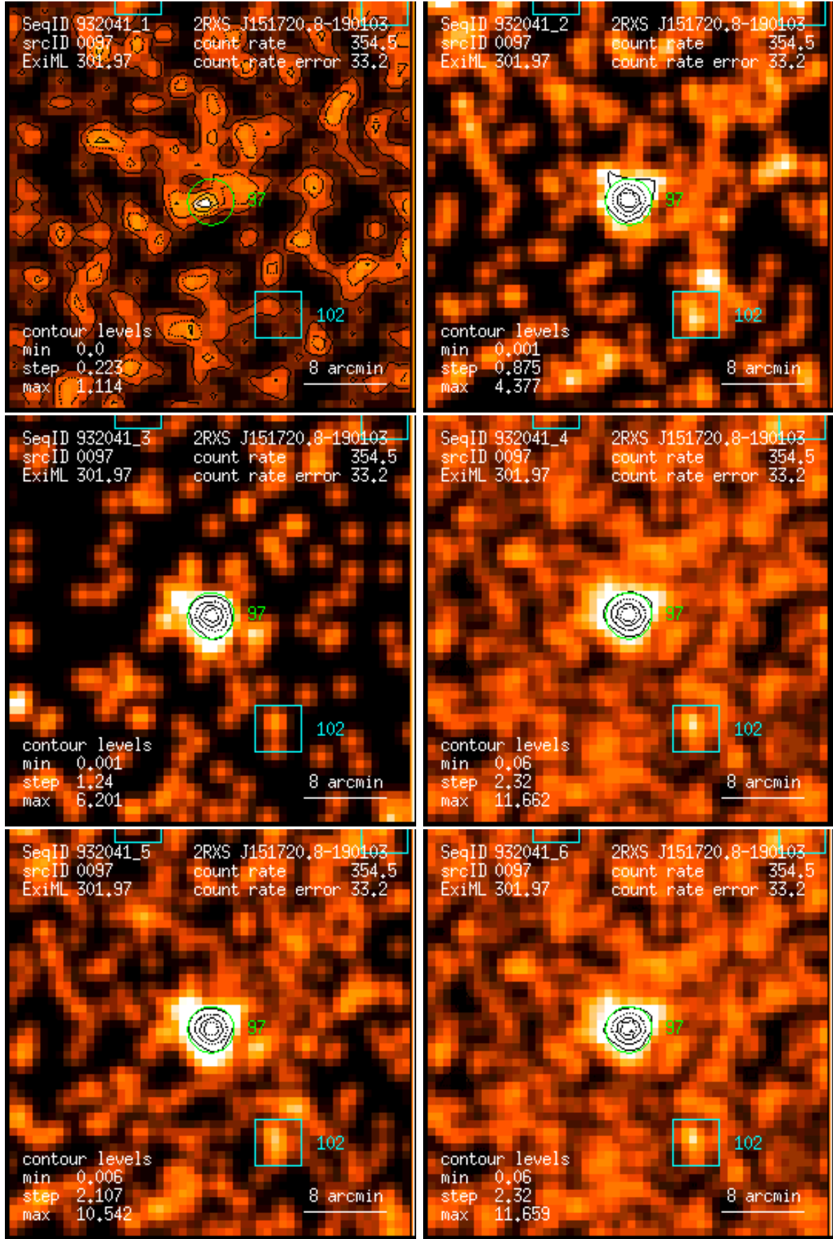
Figure 97: RASS 932041: detection 0097: band rate images, Gaussian filter: (1) PSPC channels 11 – 41, (2) 52 – 90, (3) 91 – 201, (4) 11 – 235, (5) 52 – 201, (6) 11 – 201. Broad band rates in counts/ks. Band rate contour levels in counts/ks/arcmin 2 .
