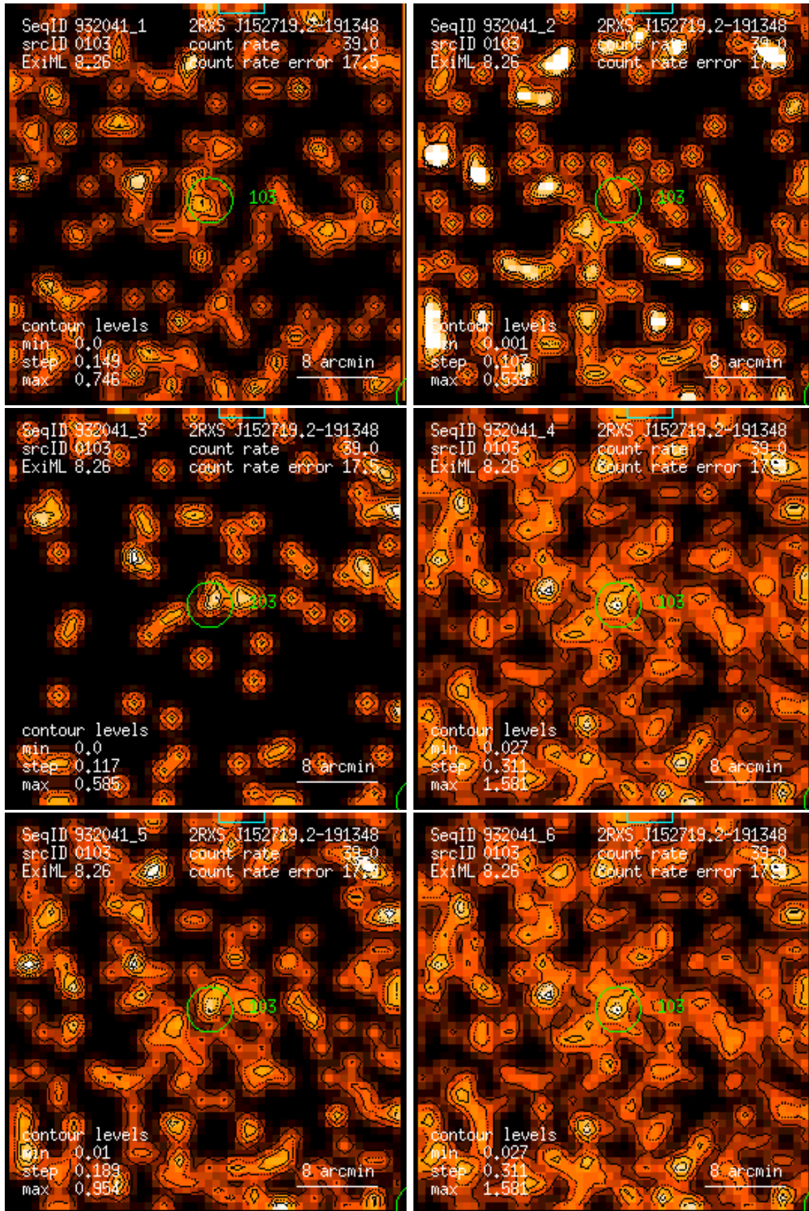
Figure 103: RASS 932041: detection 0103: band rate images, Gaussian filter: (1) PSPC channels 11 – 41, (2) 52 – 90, (3) 91 – 201, (4) 11 – 235, (5) 52 – 201, (6) 11 – 201. Broad band rates in counts/ks. Band rate contour levels in counts/ks/arcmin 2 .
