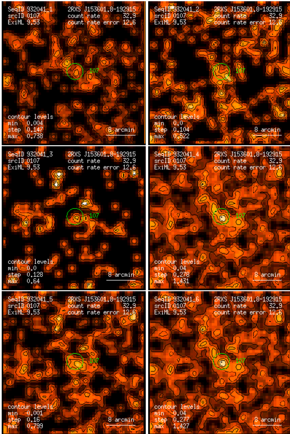
Figure 107: RASS 932041: detection 0107: band rate images, Gaussian filter: (1) PSPC channels 11 – 41, (2) 52 – 90, (3) 91 – 201, (4) 11 – 235, (5) 52 – 201, (6) 11 – 201. Broad band rates in counts/ks. Band rate contour levels in counts/ks/arcmin 2 .
