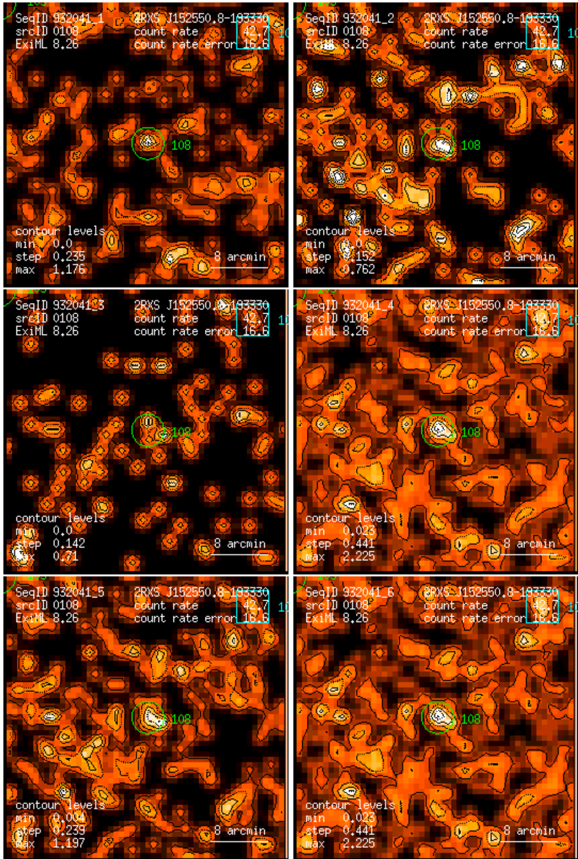
Figure 108: RASS 932041: detection 0108: band rate images, Gaussian filter: (1) PSPC channels 11 – 41, (2) 52 – 90, (3) 91 – 201, (4) 11 – 235, (5) 52 – 201, (6) 11 – 201. Broad band rates in counts/ks. Band rate contour levels in counts/ks/arcmin 2 .
