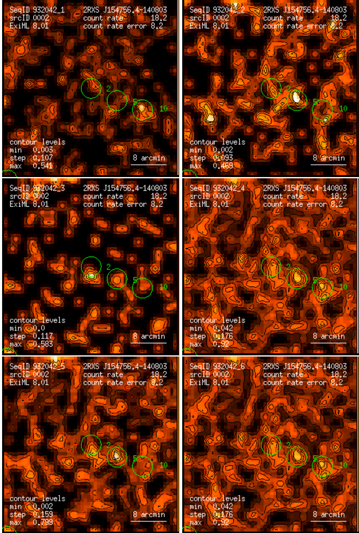
Figure 2: RASS 932042: detection 0002: band rate images, Gaussian filter: (1) PSPC channels 11 – 41, (2) 52 – 90, (3) 91 – 201, (4) 11 – 235, (5) 52 – 201, (6) 11 – 201. Broad band rates in counts/ks. Band rate contour levels in counts/ks/arcmin 2 .
