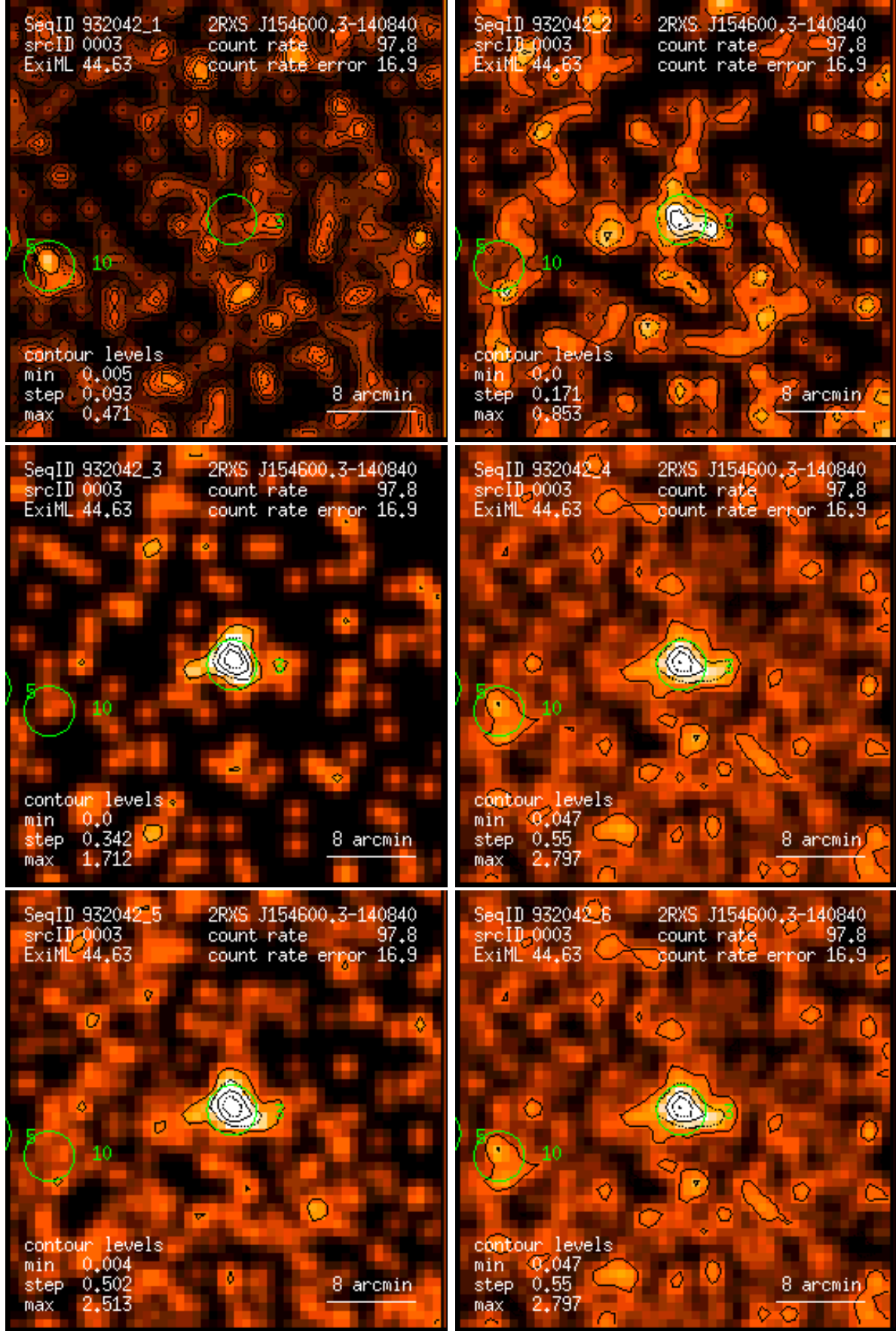
Figure 3: RASS 932042: detection 0003: band rate images, Gaussian filter: (1) PSPC channels 11 – 41, (2) 52 – 90, (3) 91 – 201, (4) 11 – 235, (5) 52 – 201, (6) 11 – 201. Broad band rates in counts/ks. Band rate contour levels in counts/ks/arcmin 2 .
