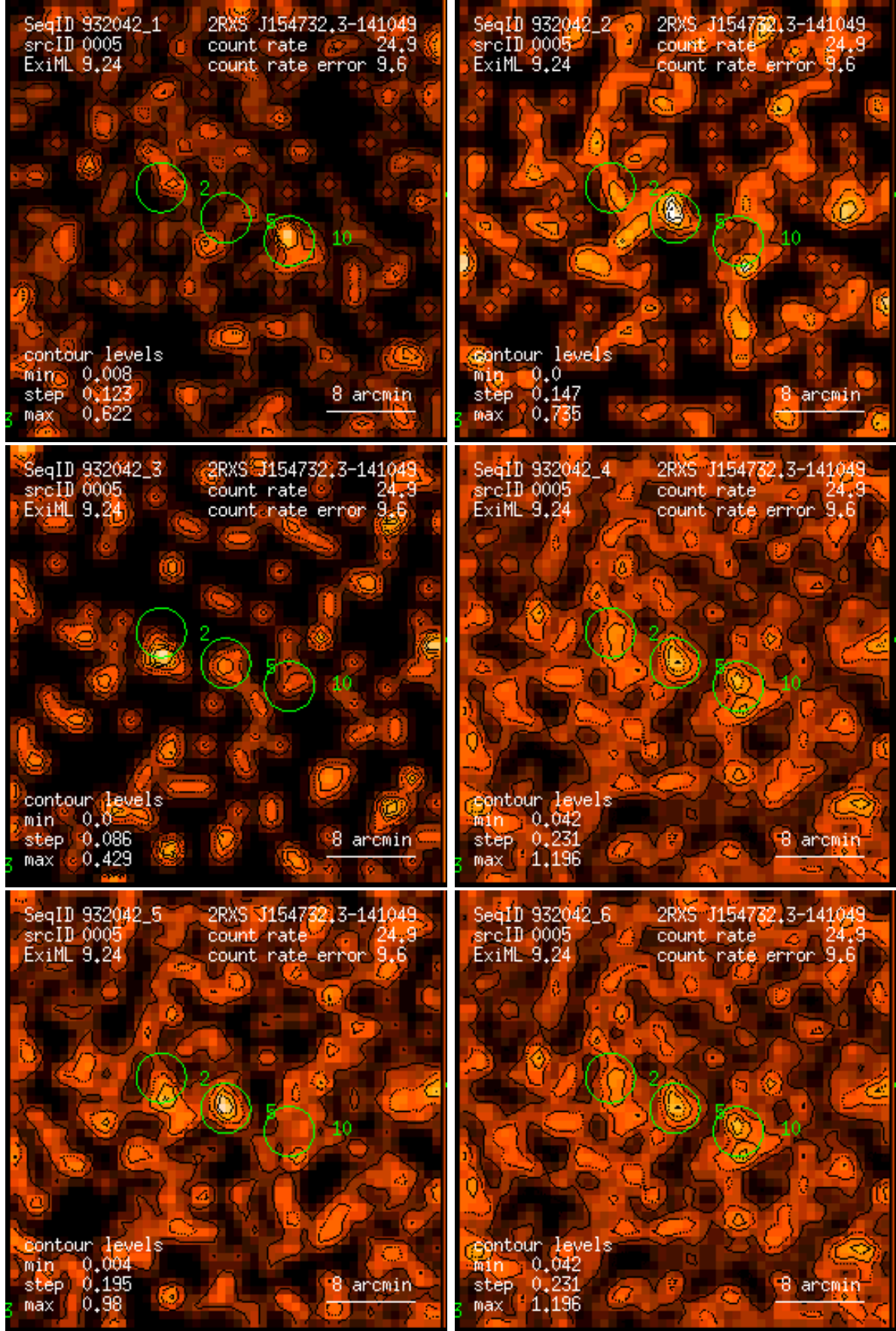
Figure 5: RASS 932042: detection 0005: band rate images, Gaussian filter: (1) PSPC channels 11 – 41, (2) 52 – 90, (3) 91 – 201, (4) 11 – 235, (5) 52 – 201, (6) 11 – 201. Broad band rates in counts/ks. Band rate contour levels in counts/ks/arcmin 2 .
