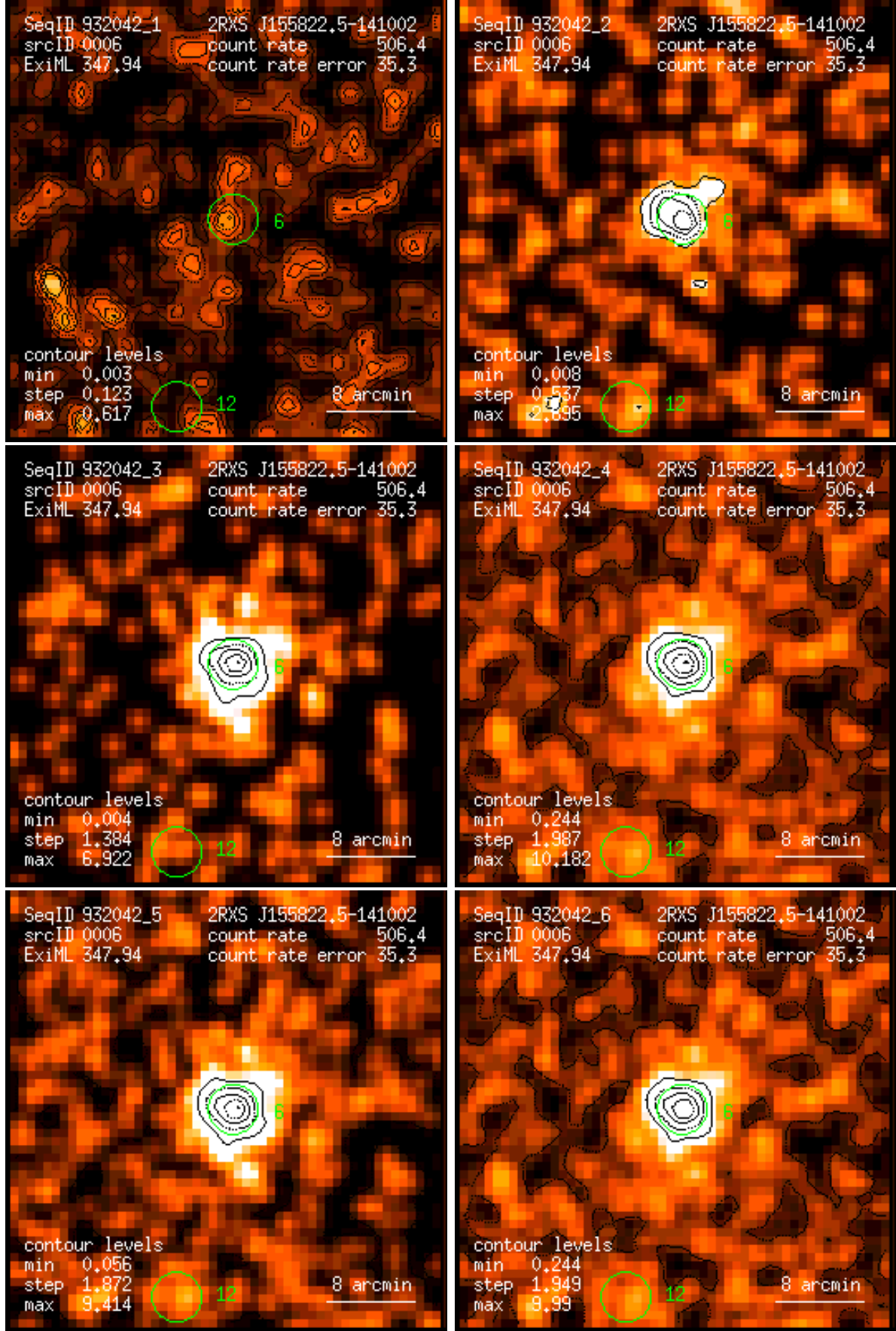
Figure 6: RASS 932042: detection 0006: band rate images, Gaussian filter: (1) PSPC channels 11 – 41, (2) 52 – 90, (3) 91 – 201, (4) 11 – 235, (5) 52 – 201, (6) 11 – 201. Broad band rates in counts/ks. Band rate contour levels in counts/ks/arcmin 2 .
