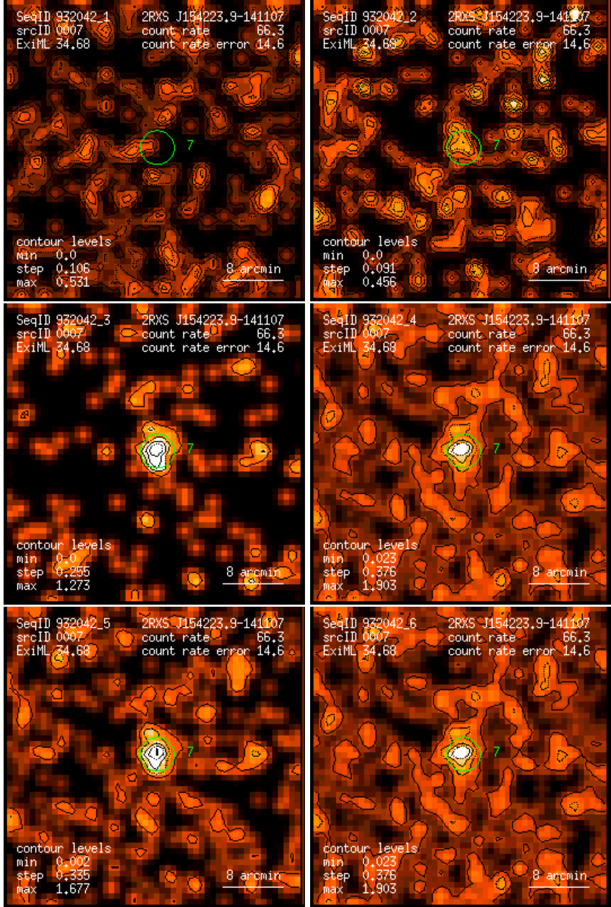
Figure 7: RASS 932042: detection 0007: band rate images, Gaussian filter: (1) PSPC channels 11 – 41, (2) 52 – 90, (3) 91 – 201, (4) 11 – 235, (5) 52 – 201, (6) 11 – 201. Broad band rates in counts/ks. Band rate contour levels in counts/ks/arcmin 2 .
