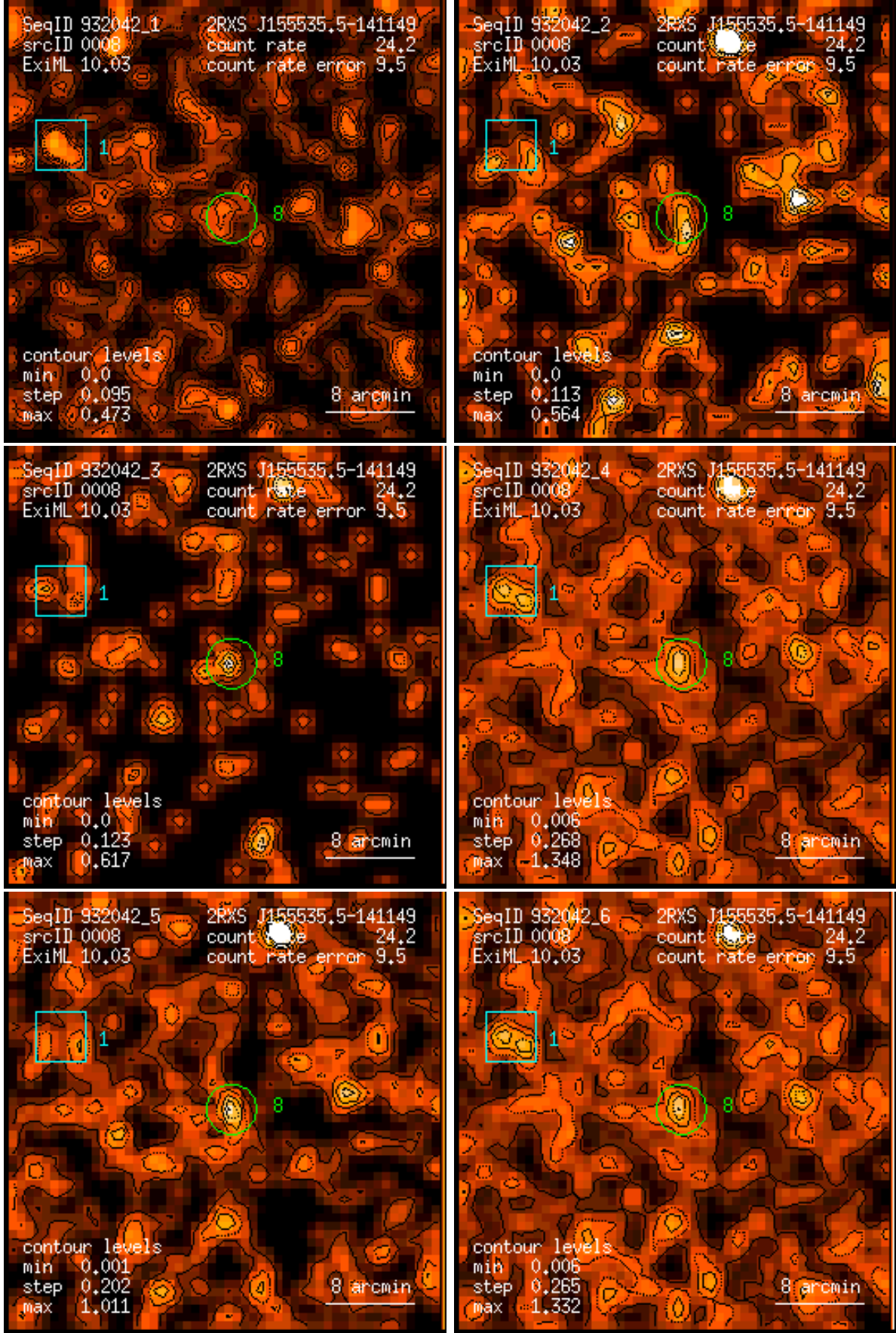
Figure 8: RASS 932042: detection 0008: band rate images, Gaussian filter: (1) PSPC channels 11 – 41, (2) 52 – 90, (3) 91 – 201, (4) 11 – 235, (5) 52 – 201, (6) 11 – 201. Broad band rates in counts/ks. Band rate contour levels in counts/ks/arcmin 2 .
