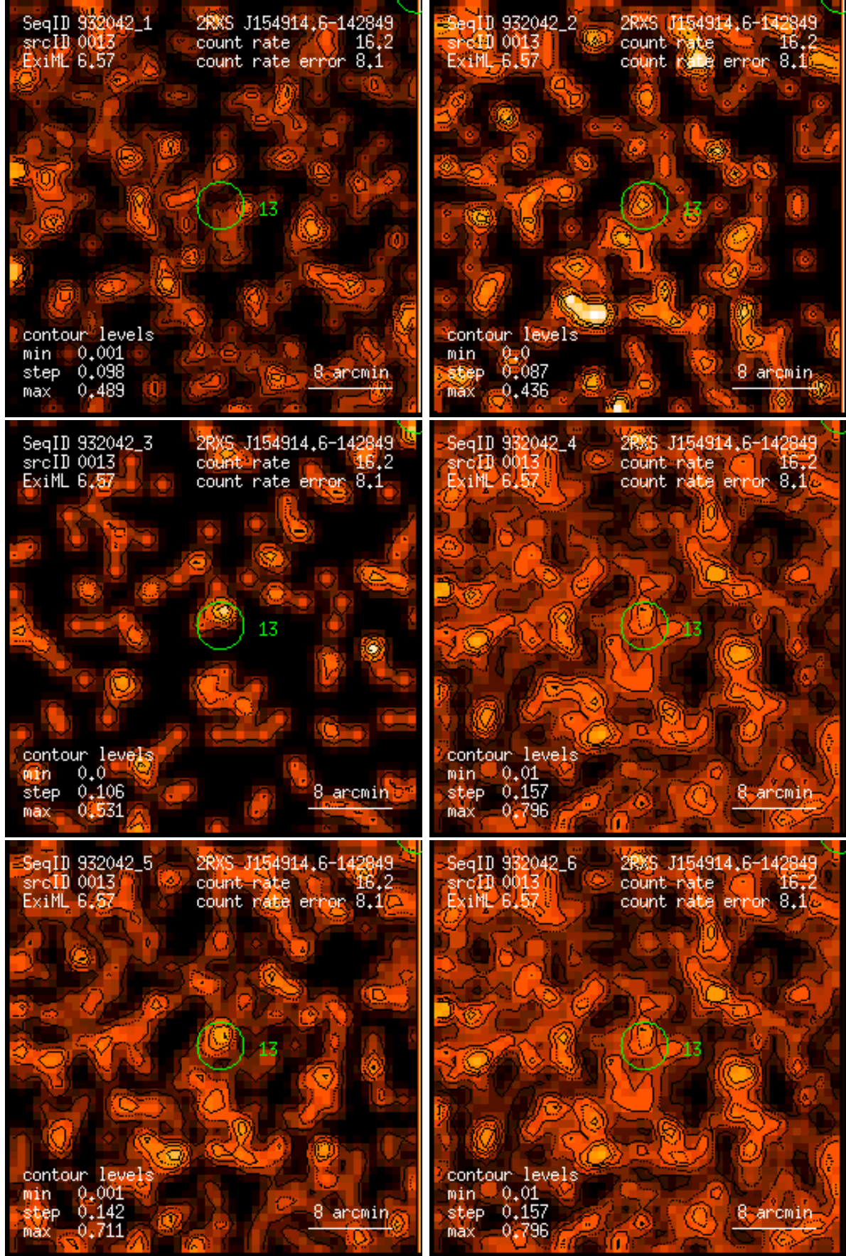
Figure 13: RASS 932042: detection 0013: band rate images, Gaussian filter: (1) PSPC channels 11 – 41, (2) 52 – 90, (3) 91 – 201, (4) 11 – 235, (5) 52 – 201, (6) 11 – 201. Broad band rates in counts/ks. Band rate contour levels in counts/ks/arcmin 2 .
