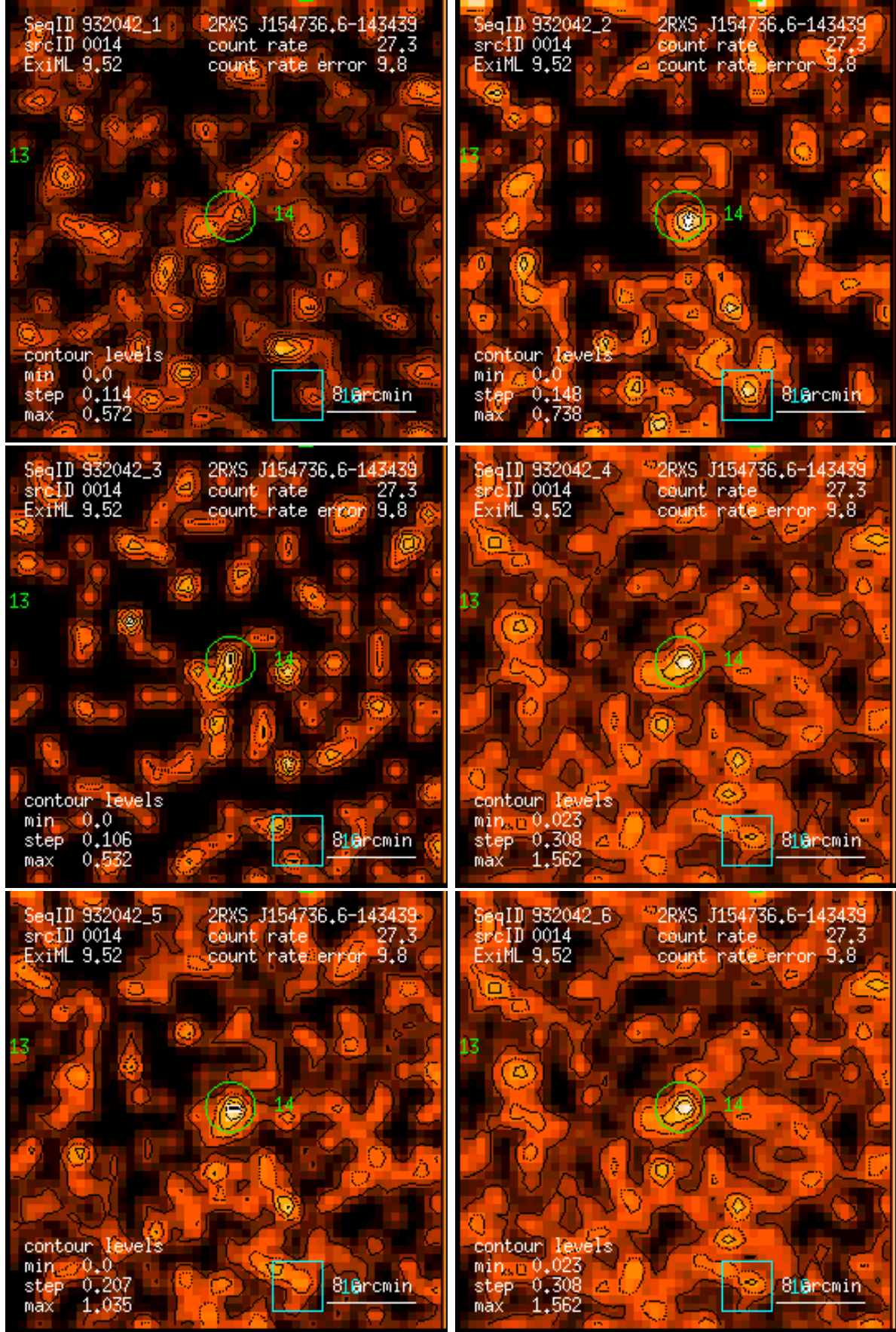
Figure 14: RASS 932042: detection 0014: band rate images, Gaussian filter: (1) PSPC channels 11 – 41, (2) 52 – 90, (3) 91 – 201, (4) 11 – 235, (5) 52 – 201, (6) 11 – 201. Broad band rates in counts/ks. Band rate contour levels in counts/ks/arcmin 2 .
