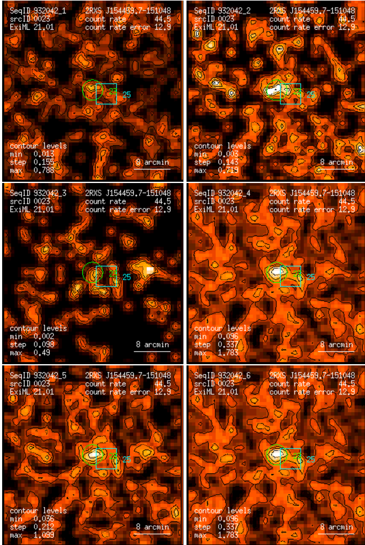
Figure 23: RASS 932042: detection 0023: band rate images, Gaussian filter: (1) PSPC channels 11 – 41, (2) 52 – 90, (3) 91 – 201, (4) 11 – 235, (5) 52 – 201, (6) 11 – 201. Broad band rates in counts/ks. Band rate contour levels in counts/ks/arcmin 2 .
