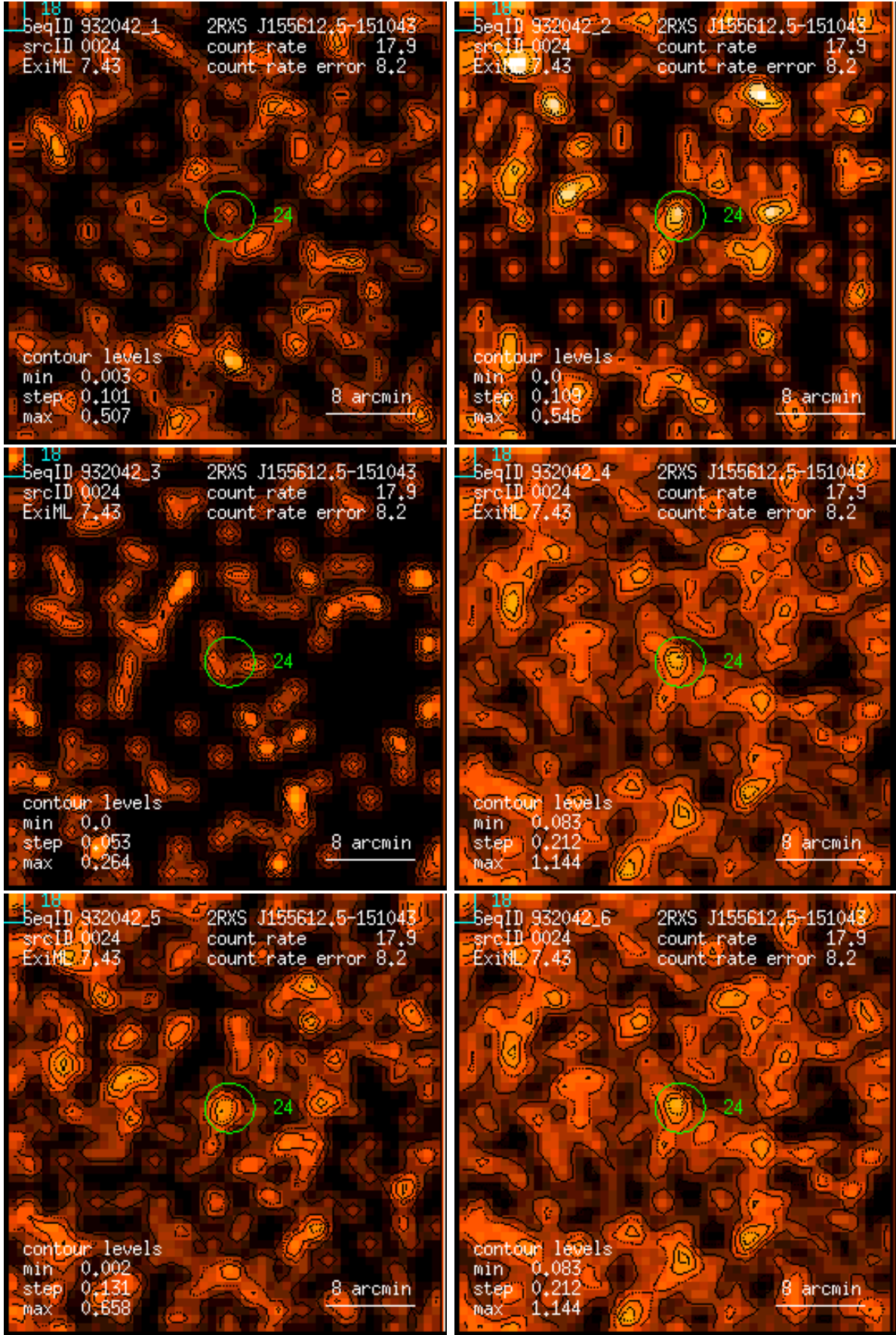
Figure 24: RASS 932042: detection 0024: band rate images, Gaussian filter: (1) PSPC channels 11 – 41, (2) 52 – 90, (3) 91 – 201, (4) 11 – 235, (5) 52 – 201, (6) 11 – 201. Broad band rates in counts/ks. Band rate contour levels in counts/ks/arcmin 2 .
