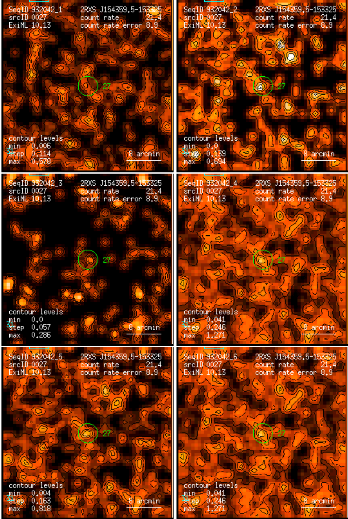
Figure 27: RASS 932042: detection 0027: band rate images, Gaussian filter: (1) PSPC channels 11 – 41, (2) 52 – 90, (3) 91 – 201, (4) 11 – 235, (5) 52 – 201, (6) 11 – 201. Broad band rates in counts/ks. Band rate contour levels in counts/ks/arcmin 2 .
