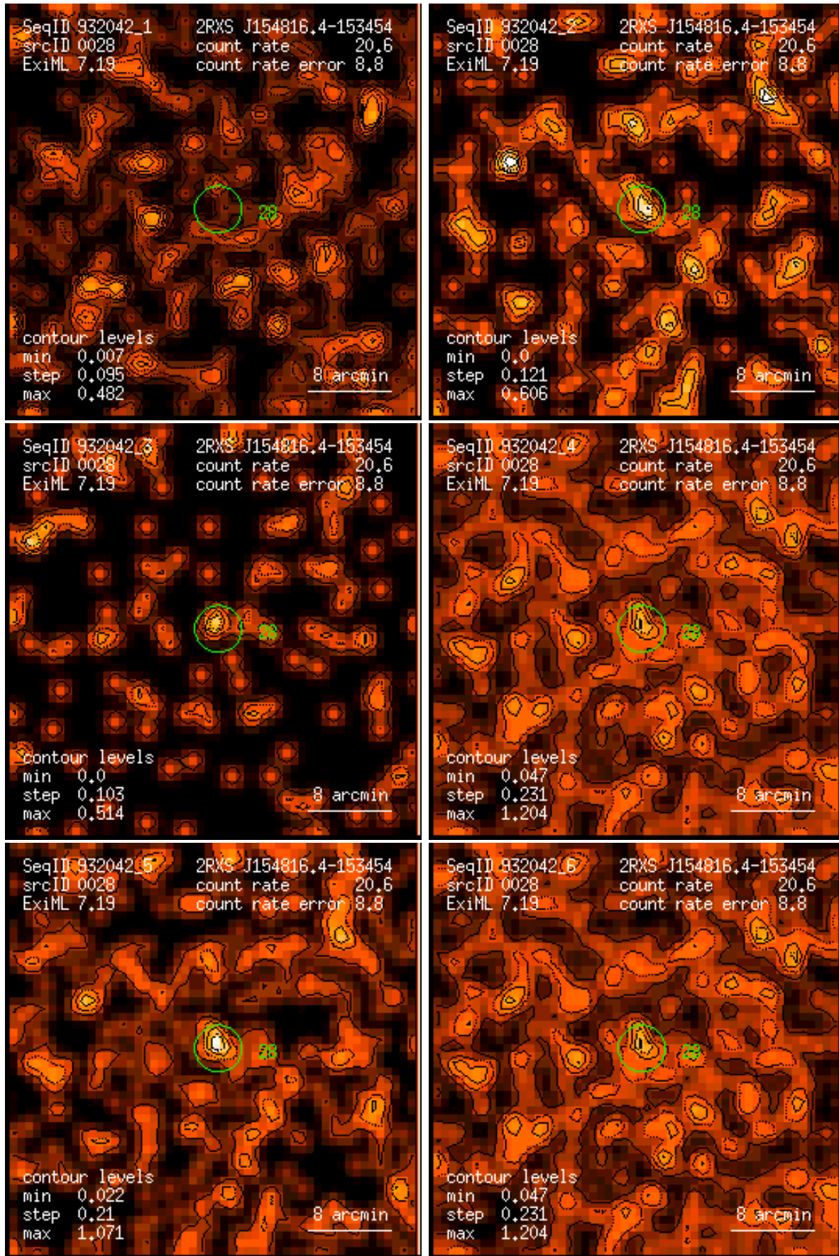
Figure 28: RASS 932042: detection 0028: band rate images, Gaussian filter: (1) PSPC channels 11 – 41, (2) 52 – 90, (3) 91 – 201, (4) 11 – 235, (5) 52 – 201, (6) 11 – 201. Broad band rates in counts/ks. Band rate contour levels in counts/ks/arcmin 2 .
