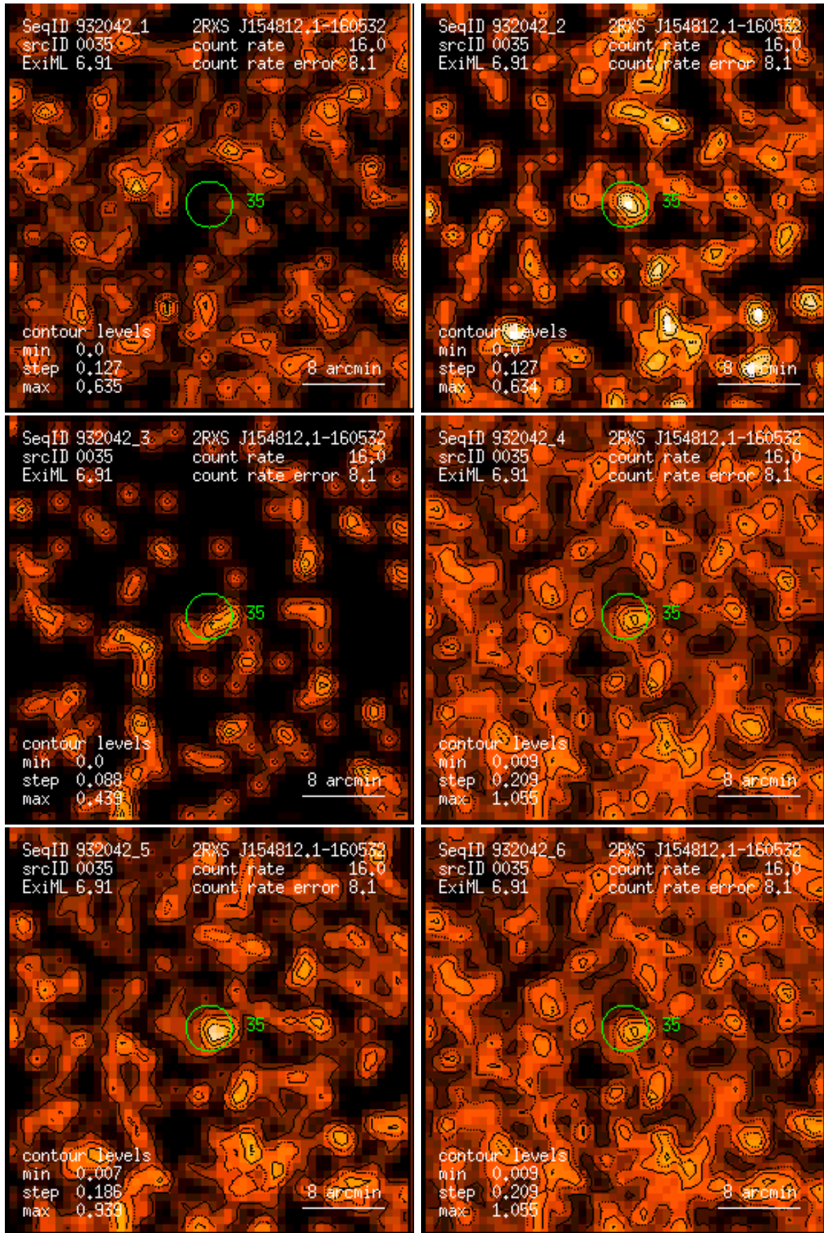
Figure 35: RASS 932042: detection 0035: band rate images, Gaussian filter: (1) PSPC channels 11 – 41, (2) 52 – 90, (3) 91 – 201, (4) 11 – 235, (5) 52 – 201, (6) 11 – 201. Broad band rates in counts/ks. Band rate contour levels in counts/ks/arcmin 2 .
