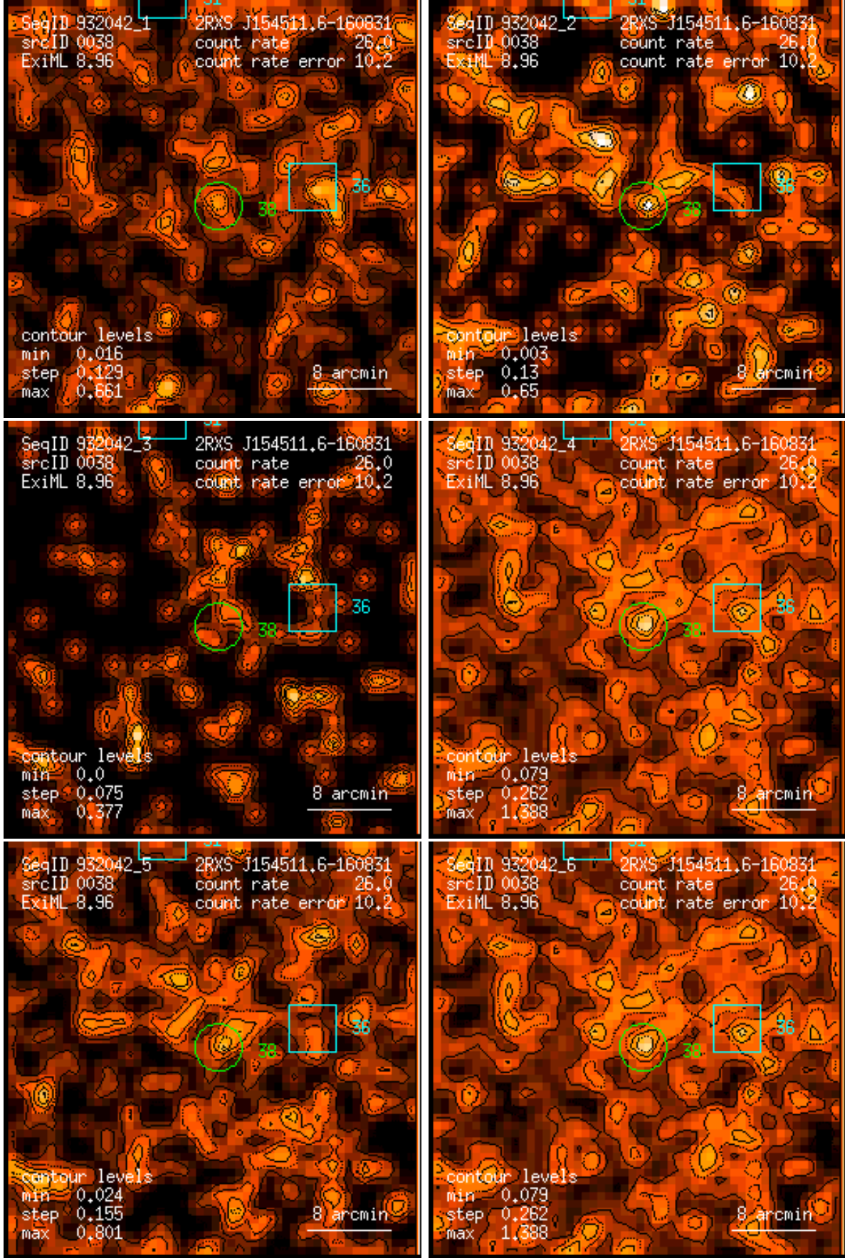
Figure 38: RASS 932042: detection 0038: band rate images, Gaussian filter: (1) PSPC channels 11 – 41, (2) 52 – 90, (3) 91 – 201, (4) 11 – 235, (5) 52 – 201, (6) 11 – 201. Broad band rates in counts/ks. Band rate contour levels in counts/ks/arcmin 2 .
