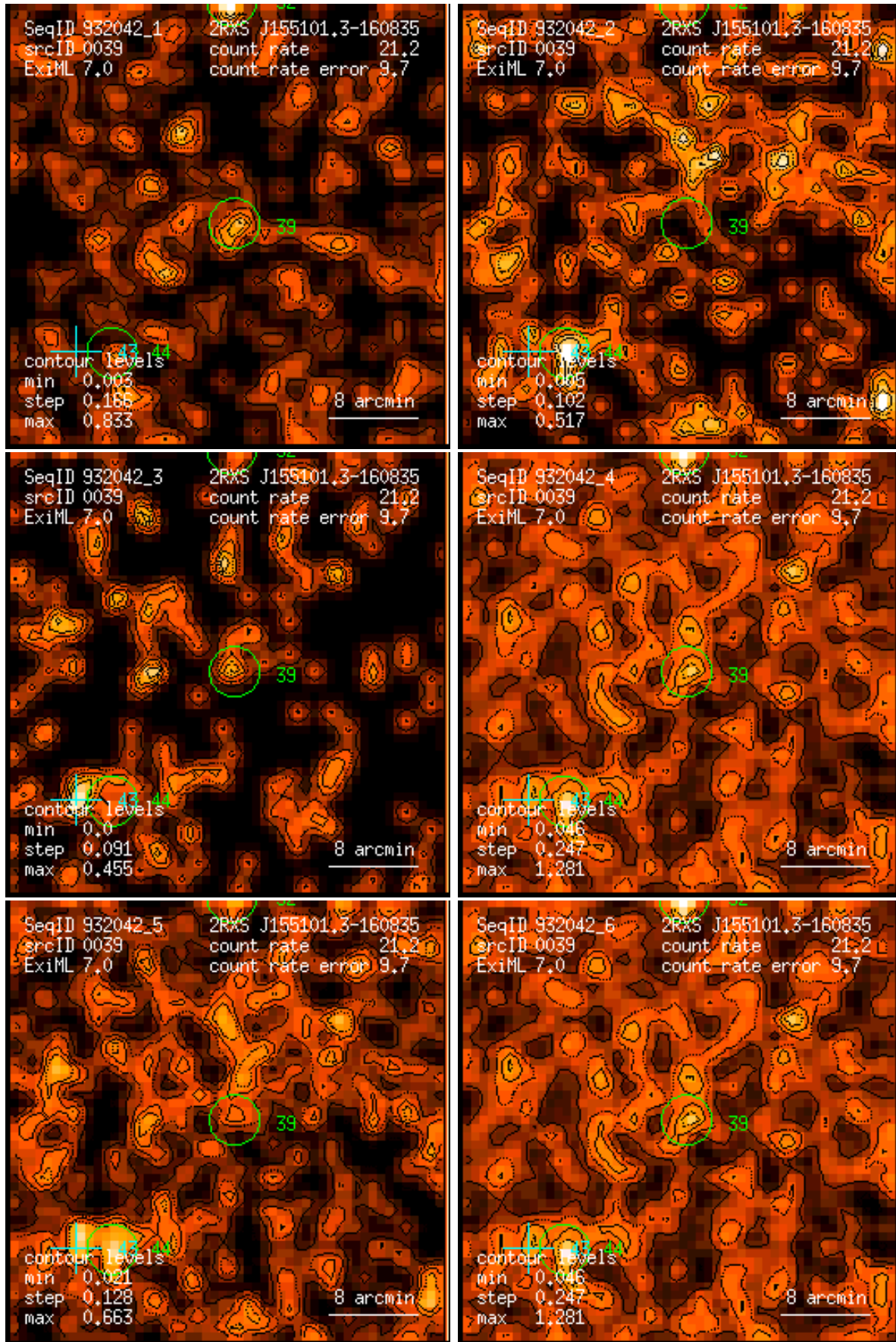
Figure 39: RASS 932042: detection 0039: band rate images, Gaussian filter: (1) PSPC channels 11 – 41, (2) 52 – 90, (3) 91 – 201, (4) 11 – 235, (5) 52 – 201, (6) 11 – 201. Broad band rates in counts/ks. Band rate contour levels in counts/ks/arcmin 2 .
