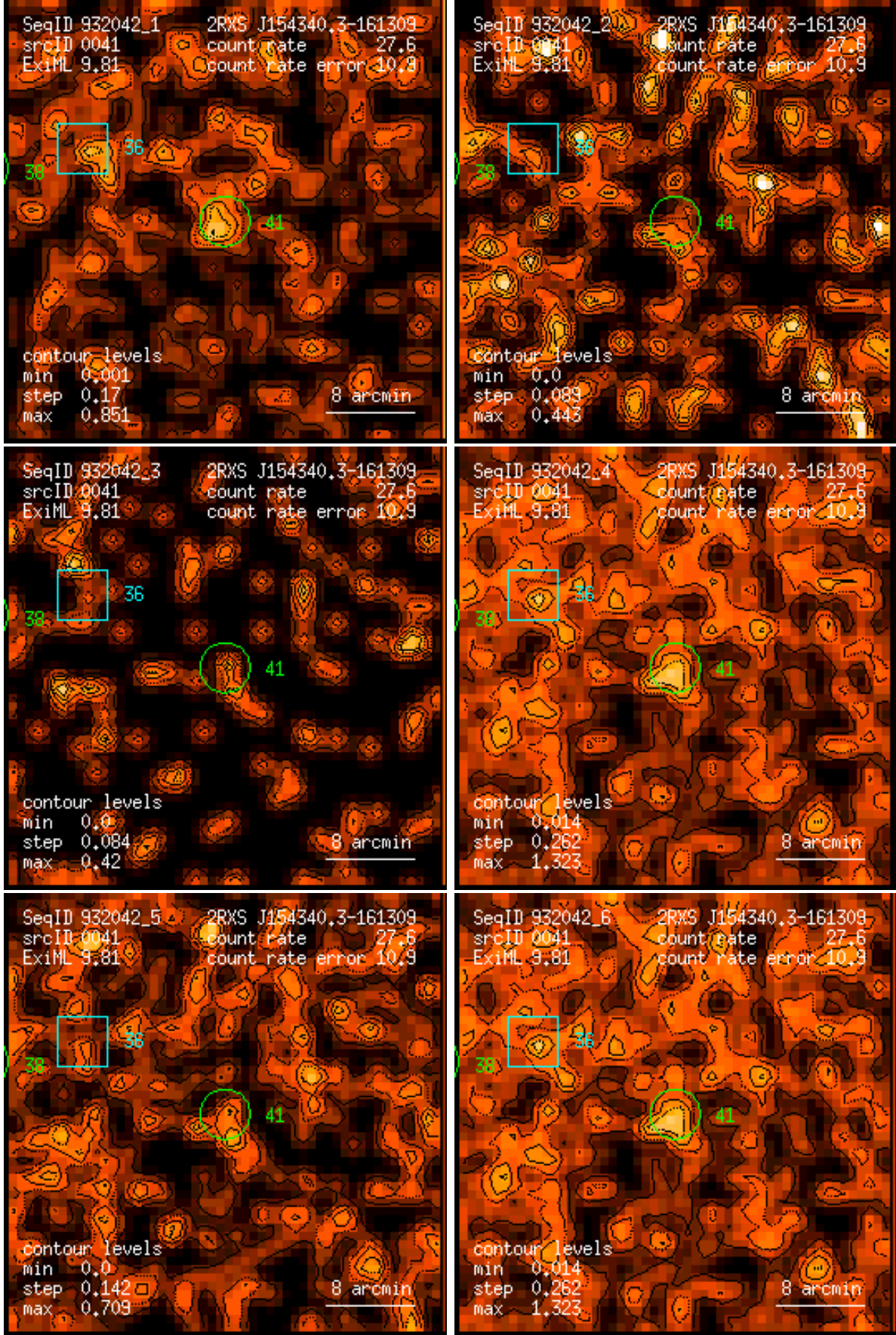
Figure 41: RASS 932042: detection 0041: band rate images, Gaussian filter: (1) PSPC channels 11 – 41, (2) 52 – 90, (3) 91 – 201, (4) 11 – 235, (5) 52 – 201, (6) 11 – 201. Broad band rates in counts/ks. Band rate contour levels in counts/ks/arcmin 2 .
