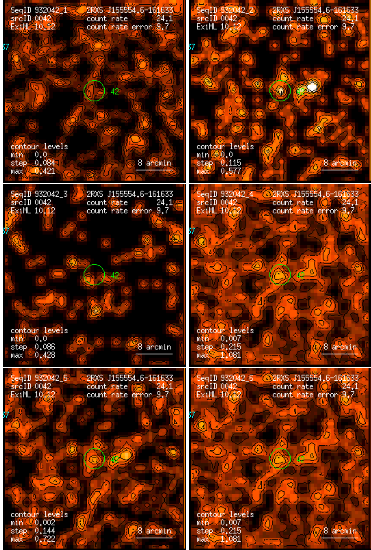
Figure 42: RASS 932042: detection 0042: band rate images, Gaussian filter: (1) PSPC channels 11 – 41, (2) 52 – 90, (3) 91 – 201, (4) 11 – 235, (5) 52 – 201, (6) 11 – 201. Broad band rates in counts/ks. Band rate contour levels in counts/ks/arcmin 2 .
