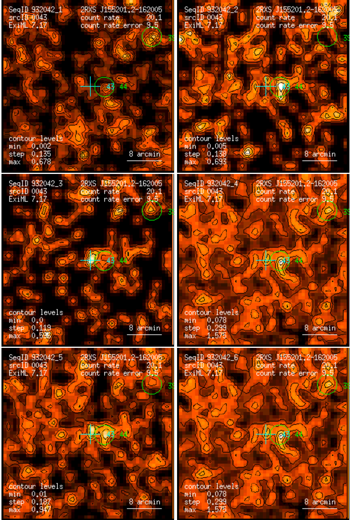
Figure 43: RASS 932042: detection 0043: band rate images, Gaussian filter: (1) PSPC channels 11 – 41, (2) 52 – 90, (3) 91 – 201, (4) 11 – 235, (5) 52 – 201, (6) 11 – 201. Broad band rates in counts/ks. Band rate contour levels in counts/ks/arcmin 2 .
