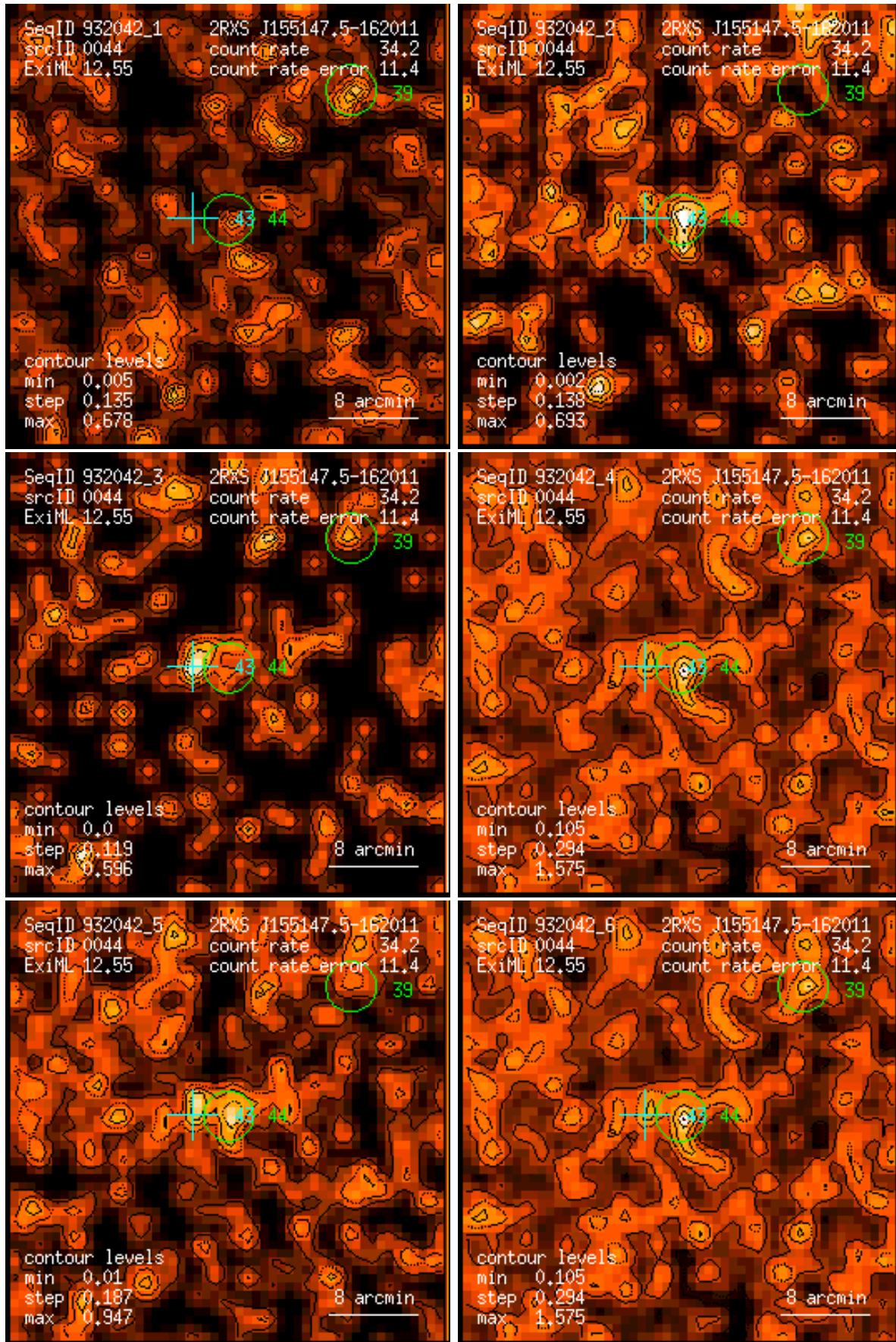
Figure 44: RASS 932042: detection 0044: band rate images, Gaussian filter: (1) PSPC channels 11 – 41, (2) 52 – 90, (3) 91 – 201, (4) 11 – 235, (5) 52 – 201, (6) 11 – 201. Broad band rates in counts/ks. Band rate contour levels in counts/ks/arcmin 2 .
