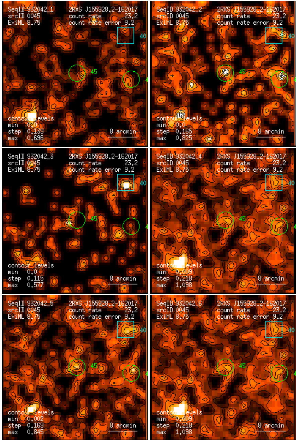
Figure 45: RASS 932042: detection 0045: band rate images, Gaussian filter: (1) PSPC channels 11 – 41, (2) 52 – 90, (3) 91 – 201, (4) 11 – 235, (5) 52 – 201, (6) 11 – 201. Broad band rates in counts/ks. Band rate contour levels in counts/ks/arcmin 2 .
