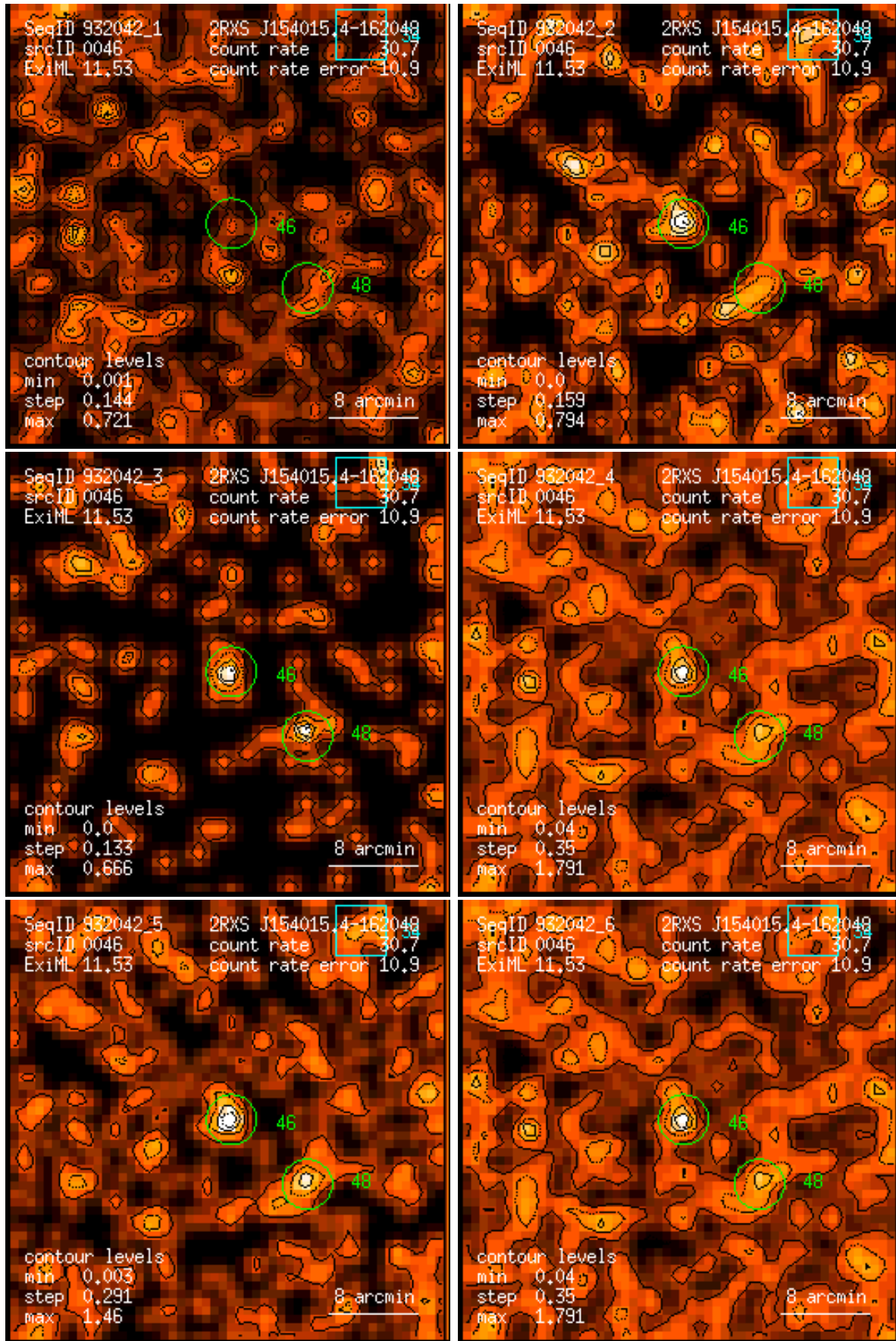
Figure 46: RASS 932042: detection 0046: band rate images, Gaussian filter: (1) PSPC channels 11 – 41, (2) 52 – 90, (3) 91 – 201, (4) 11 – 235, (5) 52 – 201, (6) 11 – 201. Broad band rates in counts/ks. Band rate contour levels in counts/ks/arcmin 2 .
