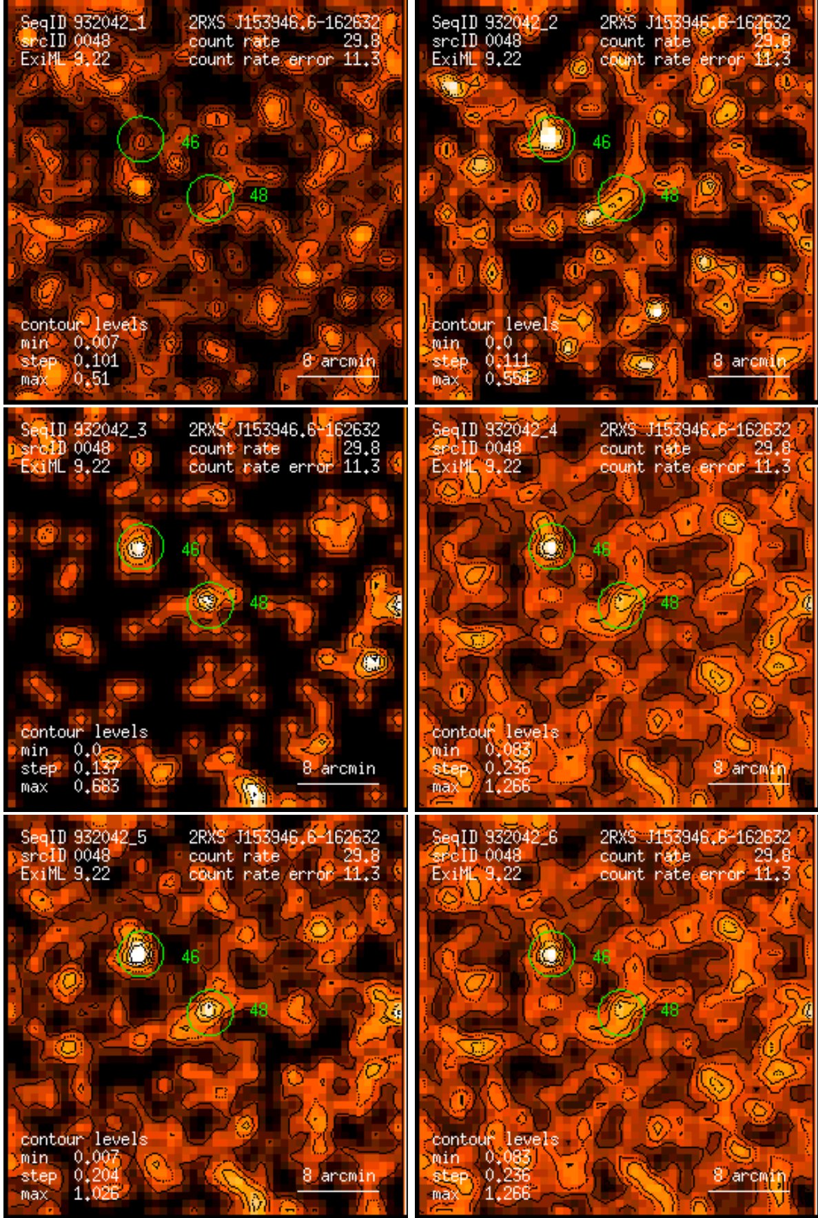
Figure 48: RASS 932042: detection 0048: band rate images, Gaussian filter: (1) PSPC channels 11 – 41, (2) 52 – 90, (3) 91 – 201, (4) 11 – 235, (5) 52 – 201, (6) 11 – 201. Broad band rates in counts/ks. Band rate contour levels in counts/ks/arcmin 2 .
