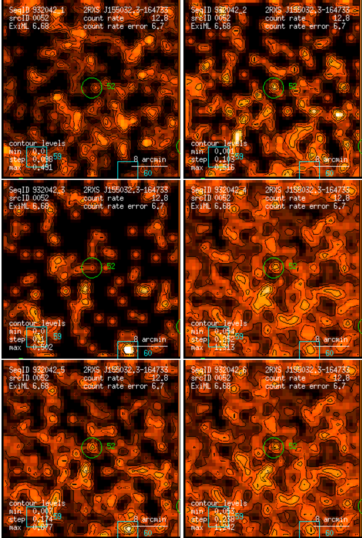
Figure 52: RASS 932042: detection 0052: band rate images, Gaussian filter: (1) PSPC channels 11 – 41, (2) 52 – 90, (3) 91 – 201, (4) 11 – 235, (5) 52 – 201, (6) 11 – 201. Broad band rates in counts/ks. Band rate contour levels in counts/ks/arcmin 2 .
