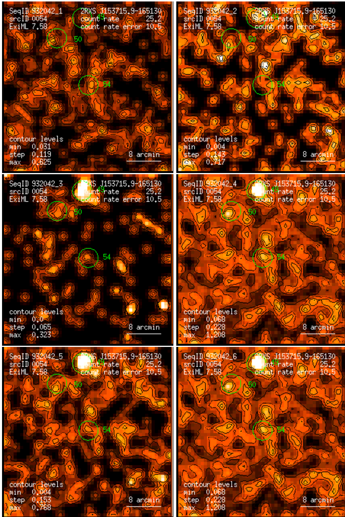
Figure 54: RASS 932042: detection 0054: band rate images, Gaussian filter: (1) PSPC channels 11 – 41, (2) 52 – 90, (3) 91 – 201, (4) 11 – 235, (5) 52 – 201, (6) 11 – 201. Broad band rates in counts/ks. Band rate contour levels in counts/ks/arcmin 2 .
