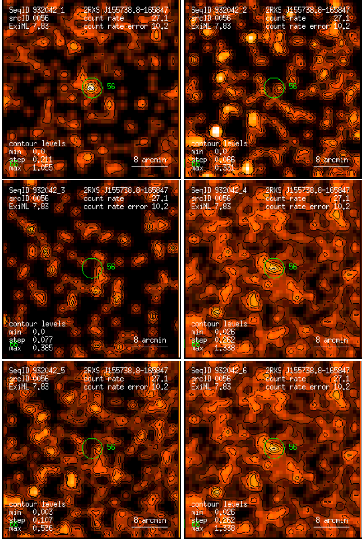
Figure 56: RASS 932042: detection 0056: band rate images, Gaussian filter: (1) PSPC channels 11 – 41, (2) 52 – 90, (3) 91 – 201, (4) 11 – 235, (5) 52 – 201, (6) 11 – 201. Broad band rates in counts/ks. Band rate contour levels in counts/ks/arcmin 2 .
