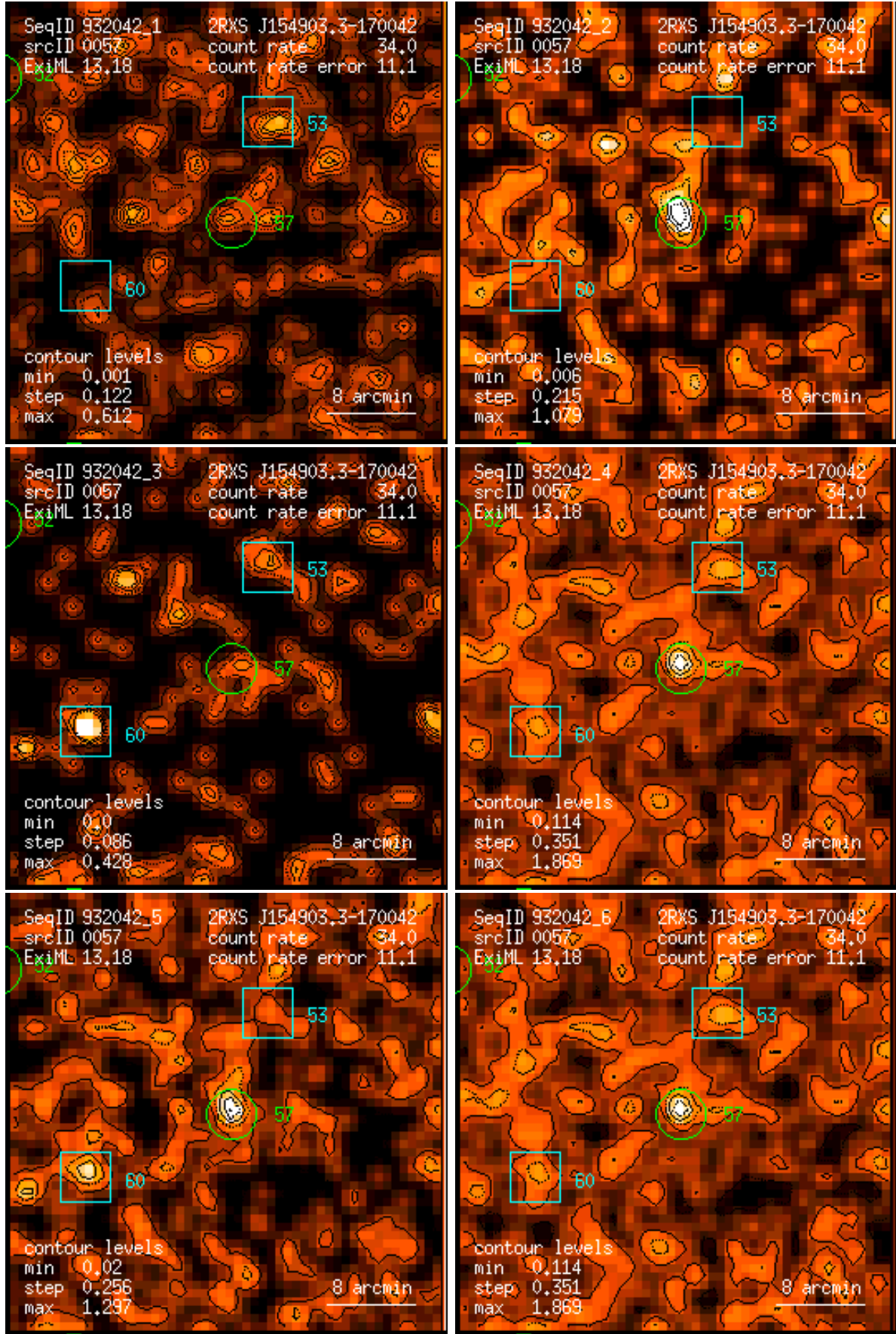
Figure 57: RASS 932042: detection 0057: band rate images, Gaussian filter: (1) PSPC channels 11 – 41, (2) 52 – 90, (3) 91 – 201, (4) 11 – 235, (5) 52 – 201, (6) 11 – 201. Broad band rates in counts/ks. Band rate contour levels in counts/ks/arcmin 2 .
