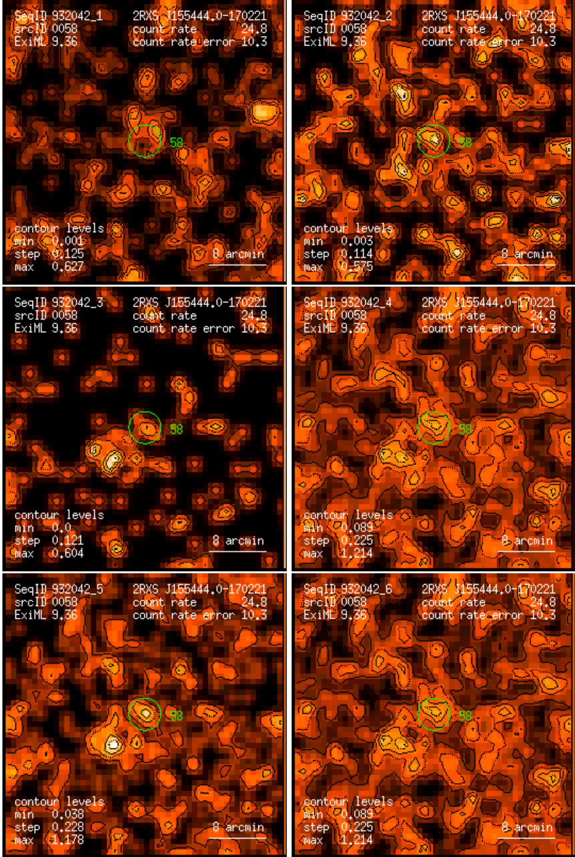
Figure 58: RASS 932042: detection 0058: band rate images, Gaussian filter: (1) PSPC channels 11 – 41, (2) 52 – 90, (3) 91 – 201, (4) 11 – 235, (5) 52 – 201, (6) 11 – 201. Broad band rates in counts/ks. Band rate contour levels in counts/ks/arcmin 2 .
