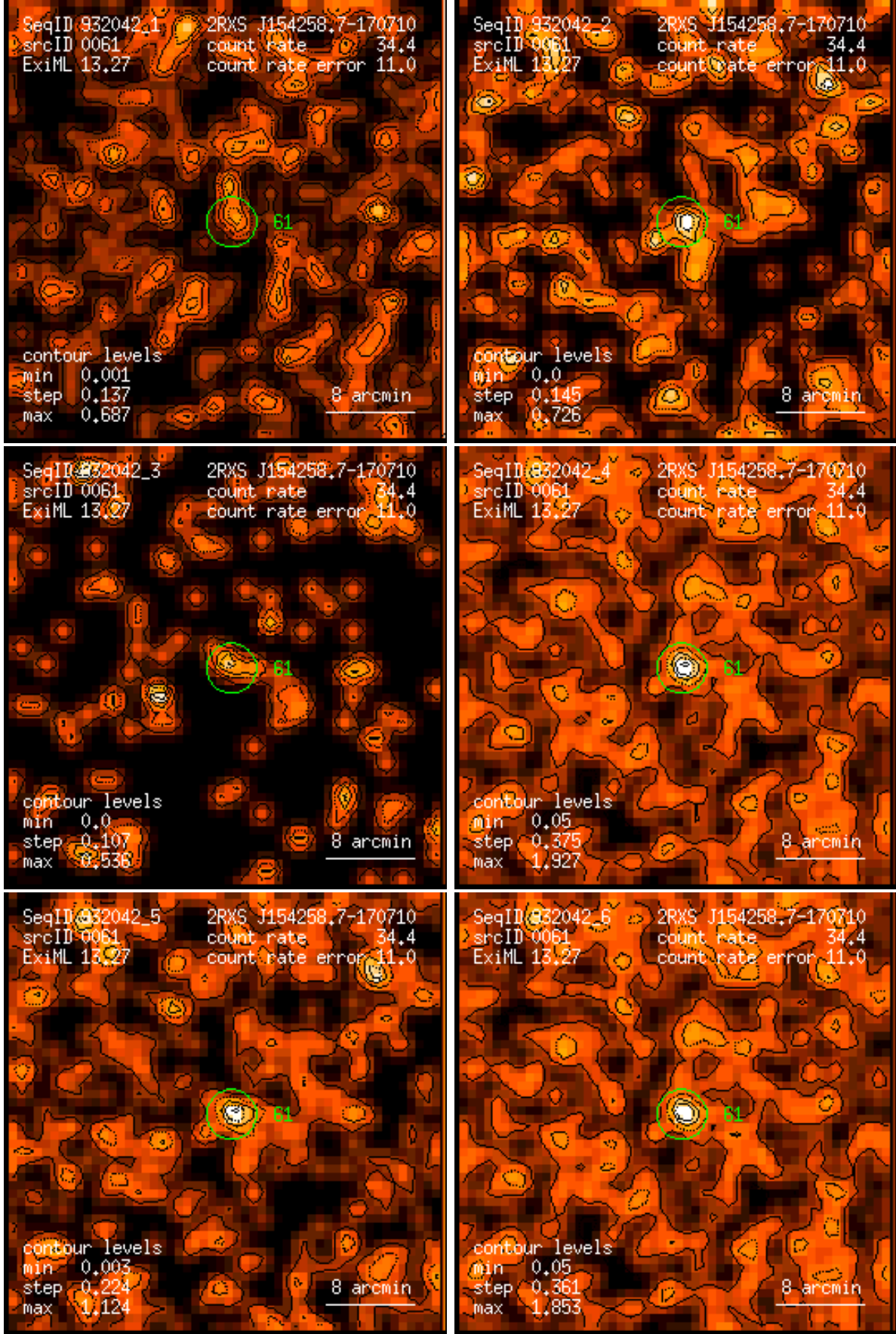
Figure 61: RASS 932042: detection 0061: band rate images, Gaussian filter: (1) PSPC channels 11 – 41, (2) 52 – 90, (3) 91 – 201, (4) 11 – 235, (5) 52 – 201, (6) 11 – 201. Broad band rates in counts/ks. Band rate contour levels in counts/ks/arcmin 2 .
