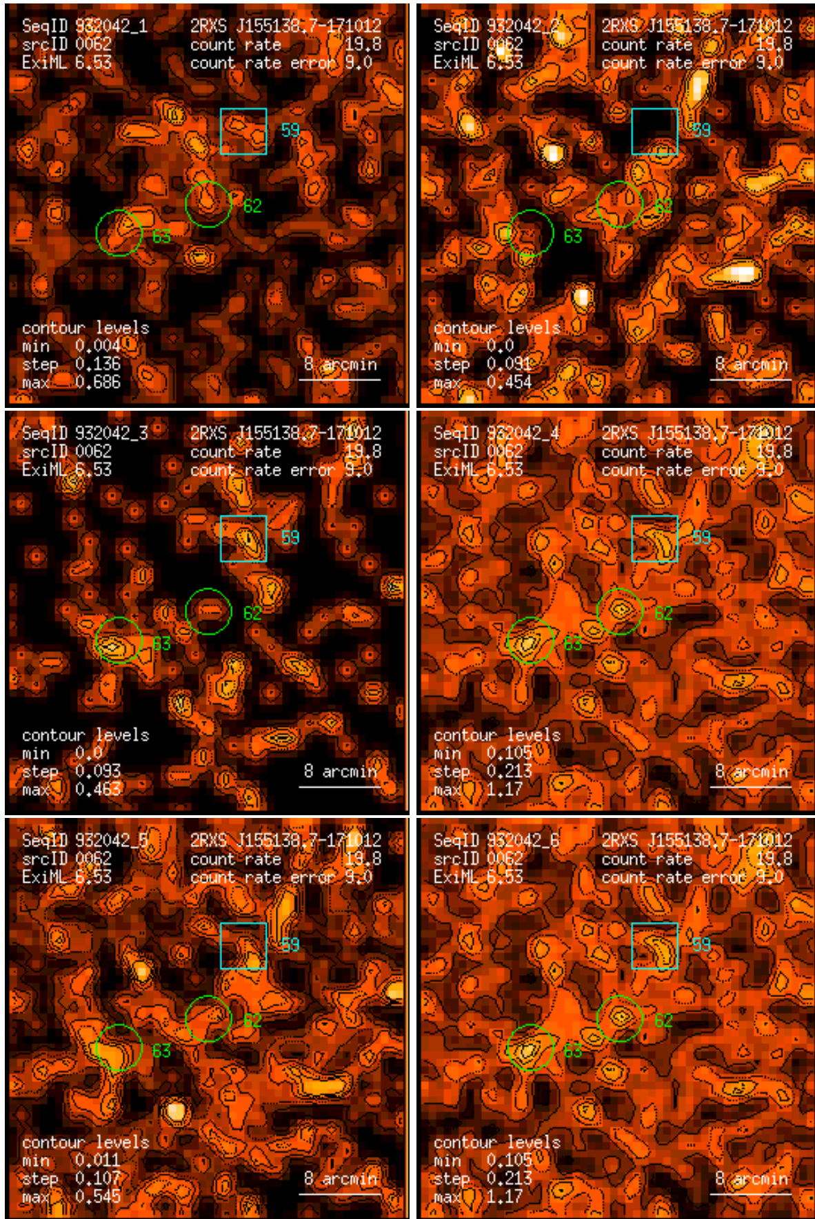
Figure 62: RASS 932042: detection 0062: band rate images, Gaussian filter: (1) PSPC channels 11 – 41, (2) 52 – 90, (3) 91 – 201, (4) 11 – 235, (5) 52 – 201, (6) 11 – 201. Broad band rates in counts/ks. Band rate contour levels in counts/ks/arcmin 2 .
