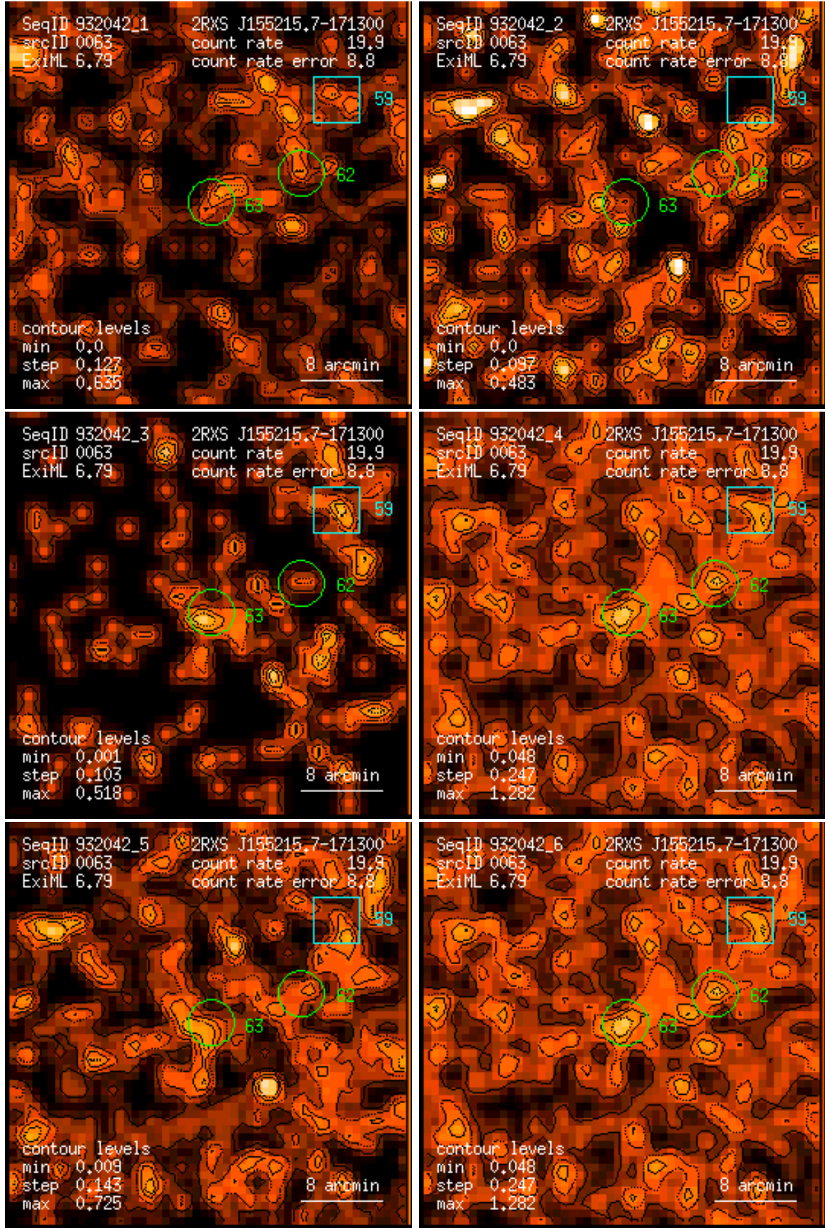
Figure 63: RASS 932042: detection 0063: band rate images, Gaussian filter: (1) PSPC channels 11 – 41, (2) 52 – 90, (3) 91 – 201, (4) 11 – 235, (5) 52 – 201, (6) 11 – 201. Broad band rates in counts/ks. Band rate contour levels in counts/ks/arcmin 2 .
