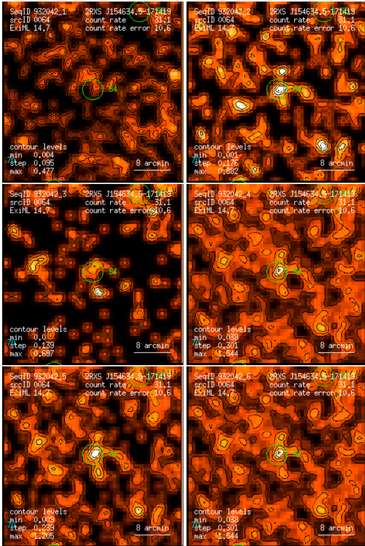
Figure 64: RASS 932042: detection 0064: band rate images, Gaussian filter: (1) PSPC channels 11 – 41, (2) 52 – 90, (3) 91 – 201, (4) 11 – 235, (5) 52 – 201, (6) 11 – 201. Broad band rates in counts/ks. Band rate contour levels in counts/ks/arcmin 2 .
