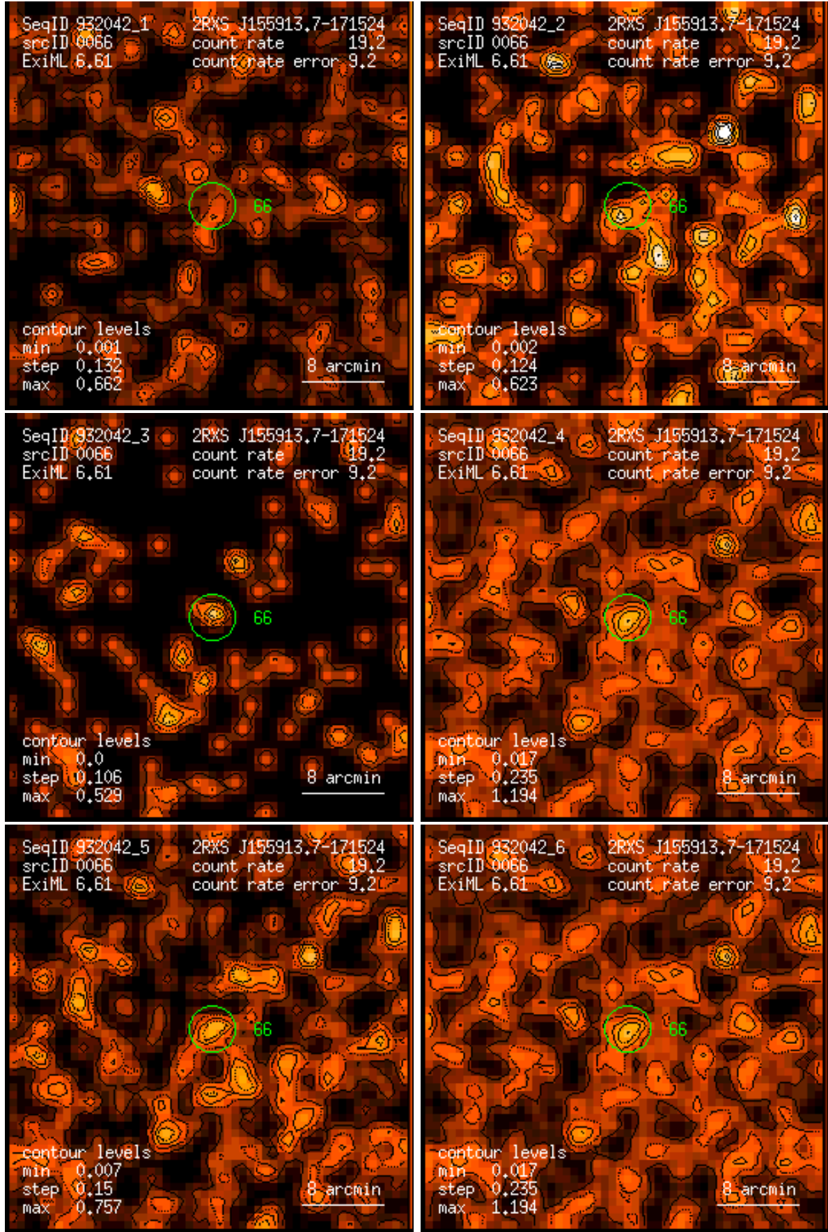
Figure 66: RASS 932042: detection 0066: band rate images, Gaussian filter: (1) PSPC channels 11 – 41, (2) 52 – 90, (3) 91 – 201, (4) 11 – 235, (5) 52 – 201, (6) 11 – 201. Broad band rates in counts/ks. Band rate contour levels in counts/ks/arcmin 2 .
