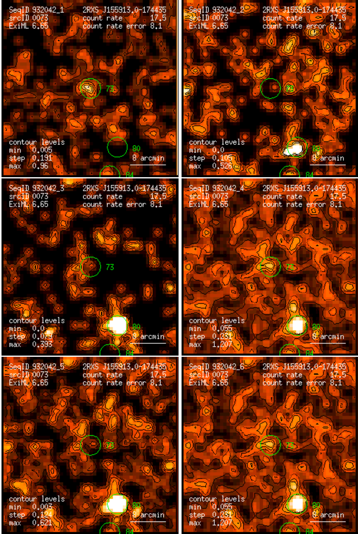
Figure 73: RASS 932042: detection 0073: band rate images, Gaussian filter: (1) PSPC channels 11 – 41, (2) 52 – 90, (3) 91 – 201, (4) 11 – 235, (5) 52 – 201, (6) 11 – 201. Broad band rates in counts/ks. Band rate contour levels in counts/ks/arcmin 2 .
