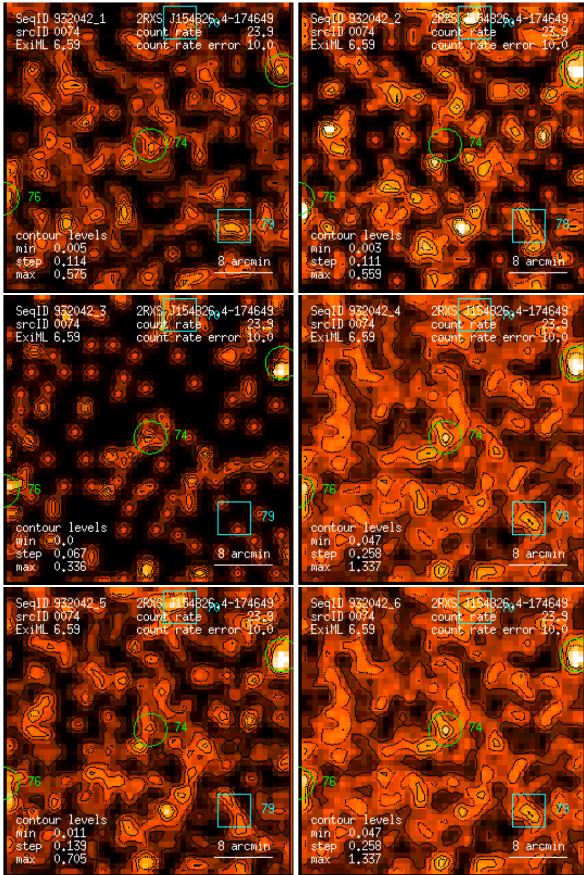
Figure 74: RASS 932042: detection 0074: band rate images, Gaussian filter: (1) PSPC channels 11 – 41, (2) 52 – 90, (3) 91 – 201, (4) 11 – 235, (5) 52 – 201, (6) 11 – 201. Broad band rates in counts/ks. Band rate contour levels in counts/ks/arcmin 2 .
