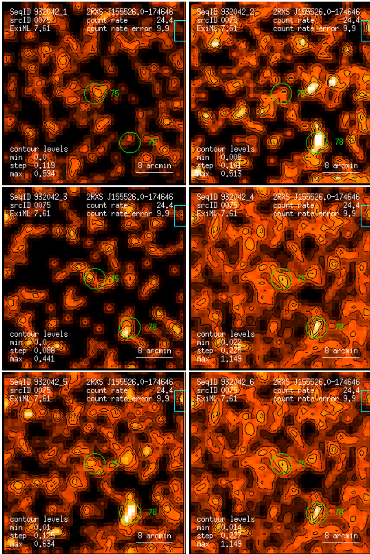
Figure 75: RASS 932042: detection 0075: band rate images, Gaussian filter: (1) PSPC channels 11 – 41, (2) 52 – 90, (3) 91 – 201, (4) 11 – 235, (5) 52 – 201, (6) 11 – 201. Broad band rates in counts/ks. Band rate contour levels in counts/ks/arcmin 2 .
