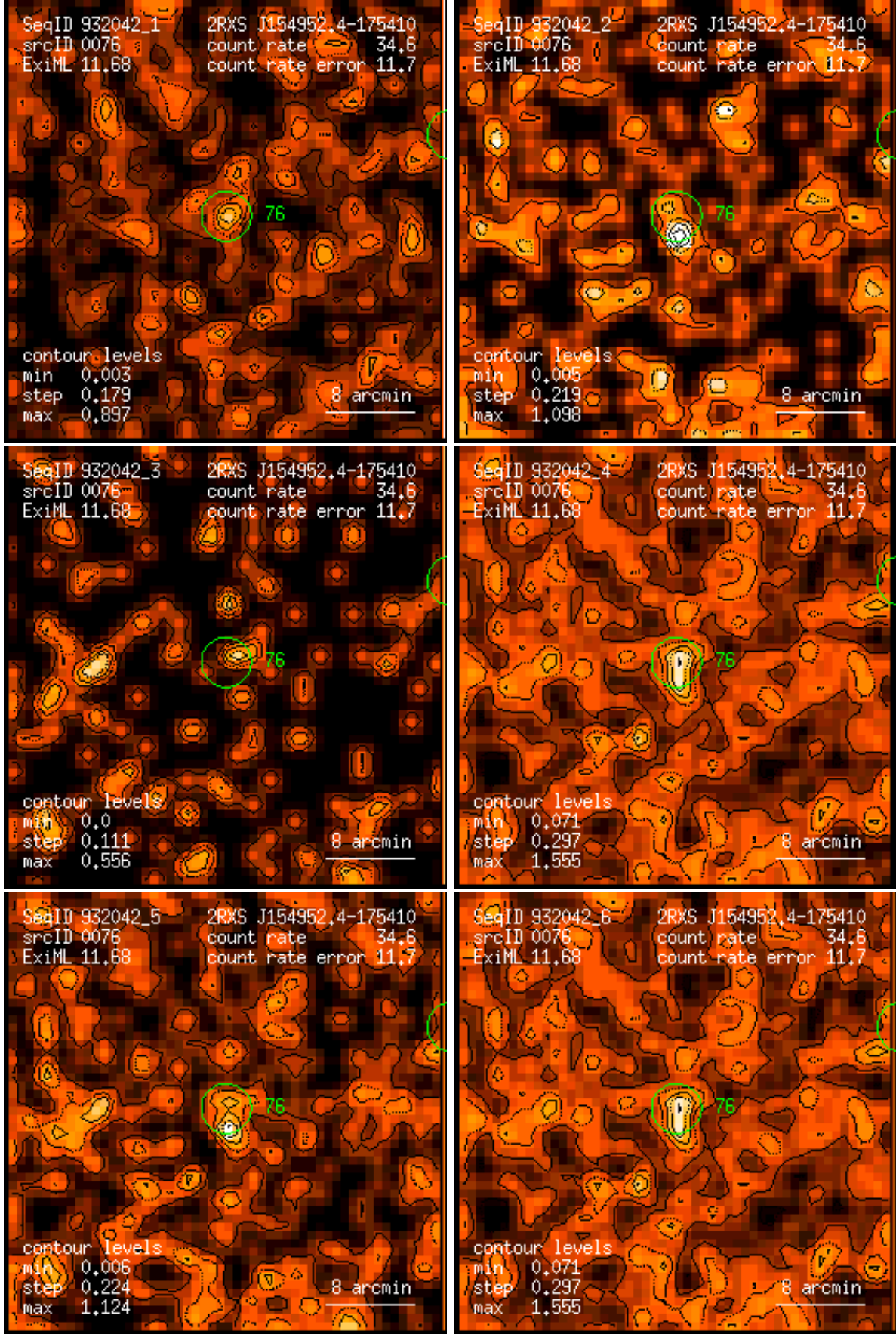
Figure 76: RASS 932042: detection 0076: band rate images, Gaussian filter: (1) PSPC channels 11 – 41, (2) 52 – 90, (3) 91 – 201, (4) 11 – 235, (5) 52 – 201, (6) 11 – 201. Broad band rates in counts/ks. Band rate contour levels in counts/ks/arcmin 2 .
